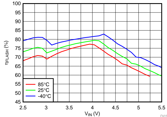
Figure 45. LED Flash Efficiency vs Input Voltage
