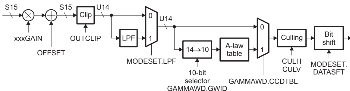
Figure 27. Output Formatter Functional Model
