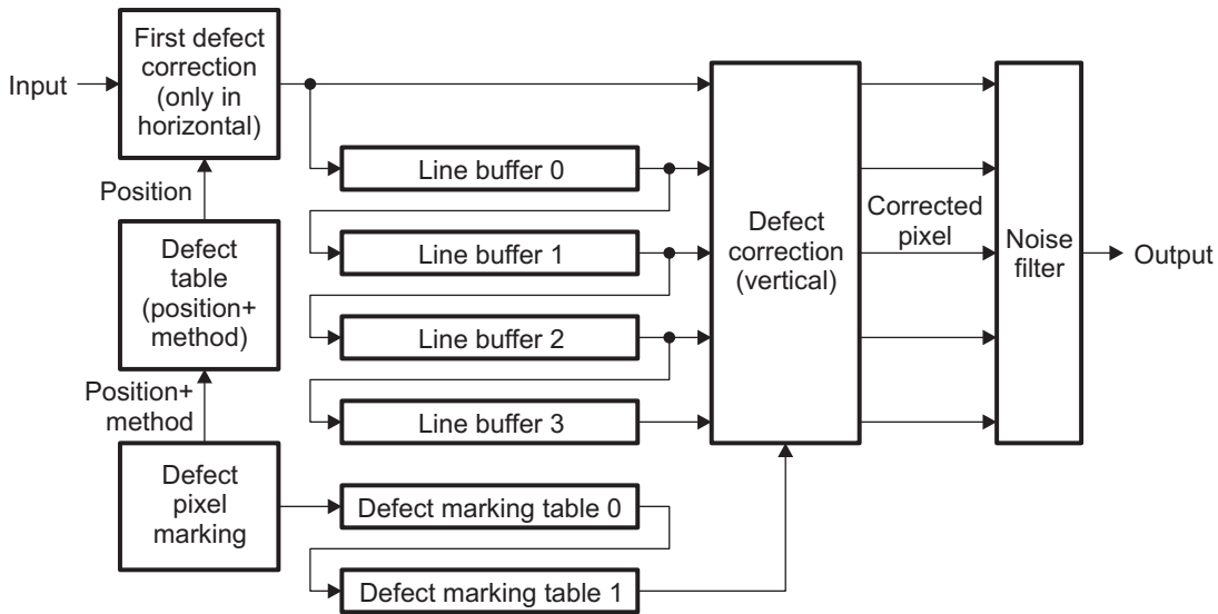
Figure 42. Defect Correction Functional Model
