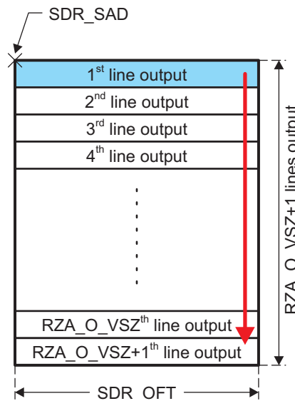
Figure 55. Linear Buffer
