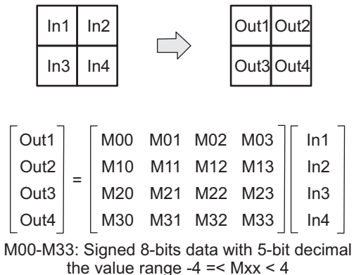
Figure 16. Color Space Converter Operation
