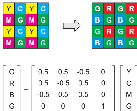
Figure 17. Color Space Converter Operation
