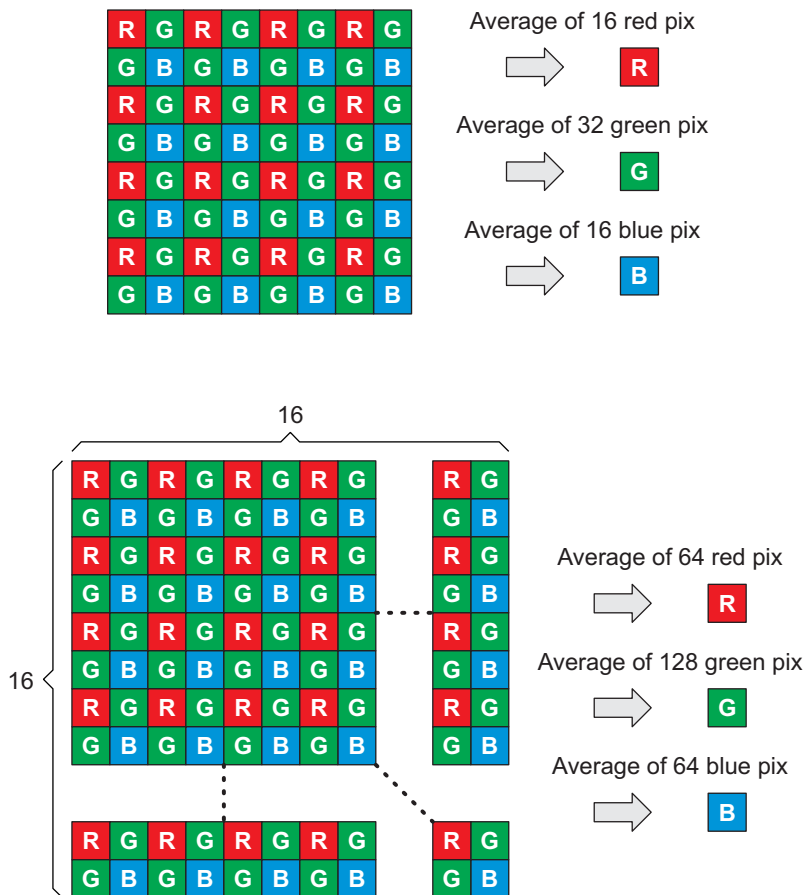
Figure 60. Boxcar Operation (8 x 8 block)
