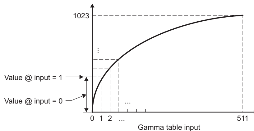
Figure 47. Example of Gamma Curve
