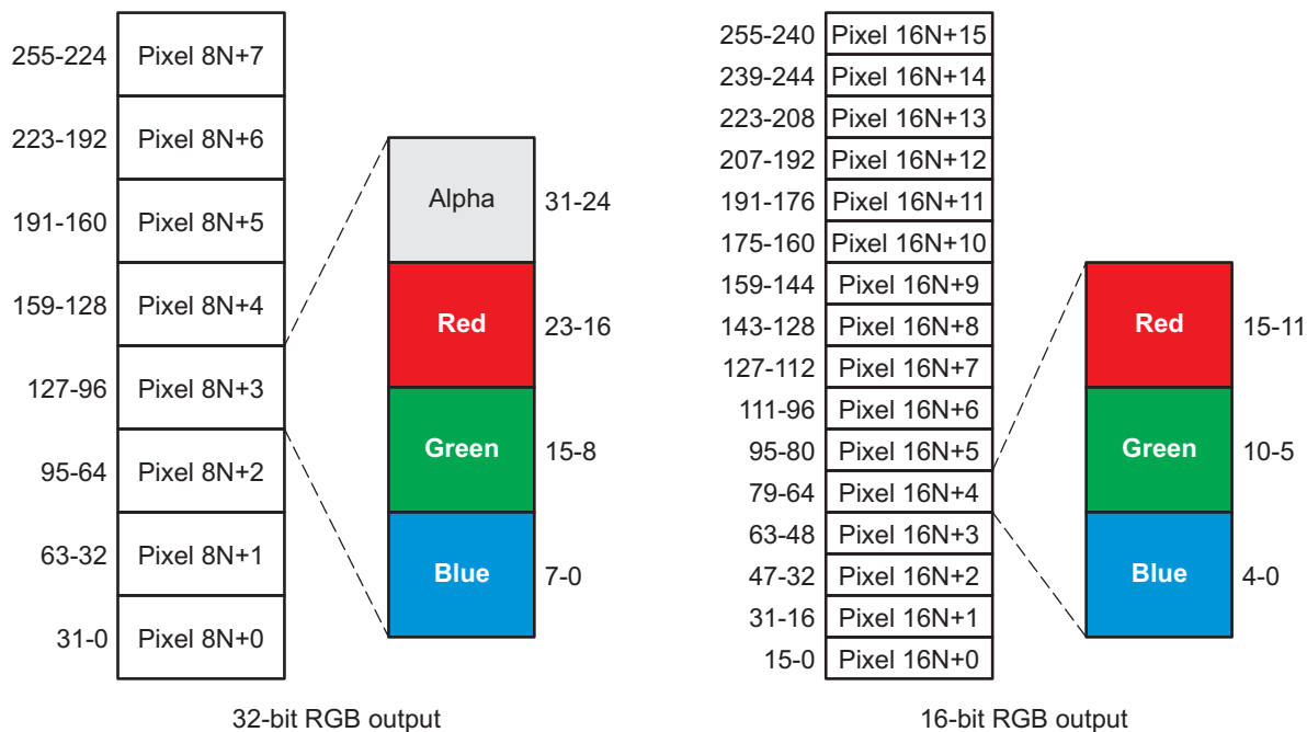
Figure 54. RGB Data Format
