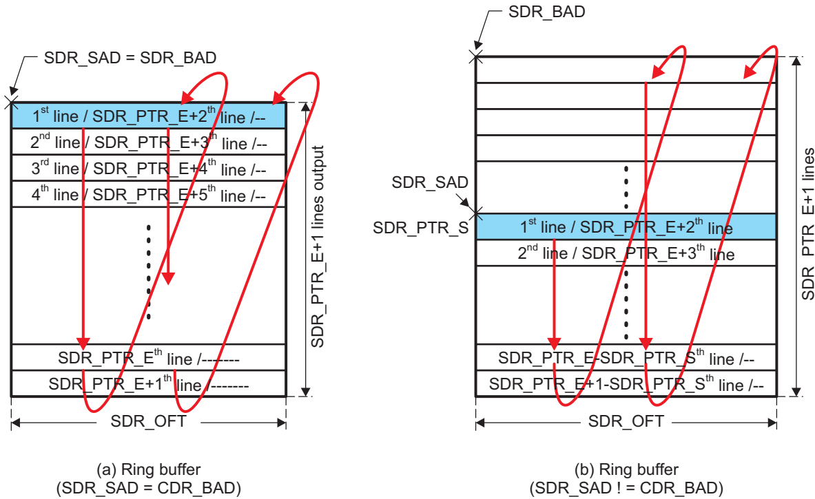
Figure 56. Ring Buffer
