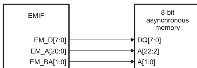
Figure 3. EMIF to 8-bit and 16-bit Memory Interfaces
