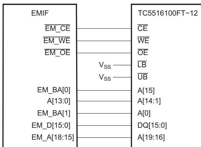
Figure 14. Connecting the EMIF to the TC55V16100FT-12
