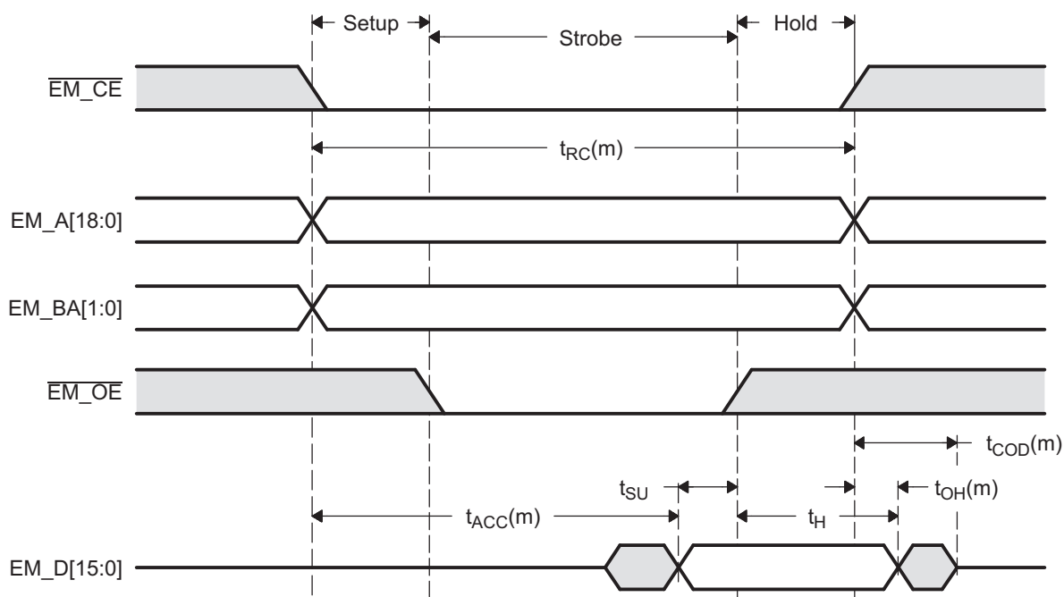
Figure 15. Timing Waveform of an ASRAM Read
