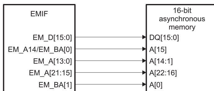
b) EMIF to 16-bit memory interface
