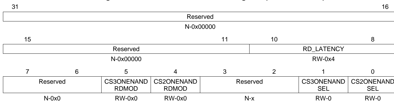
Figure 29. OneNAND Flash Control Register (ONENANDCTL)
