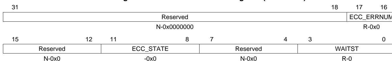
Figure 31. NAND Flash Status Register (NANDFSR)
