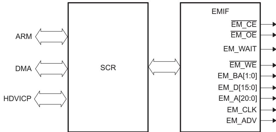
Figure 1. EMIF Functional Block Diagram
