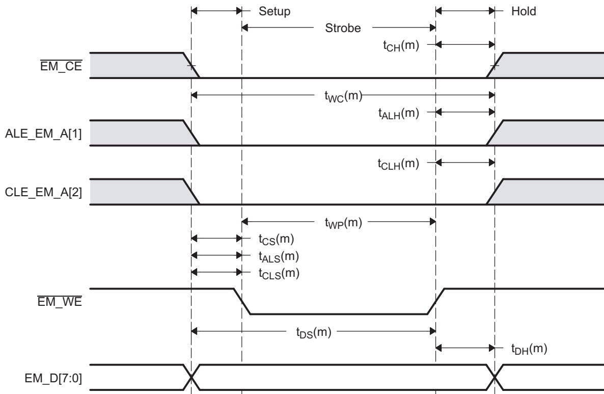
Figure 22. Timing Waveform of a NAND Flash Data Write
