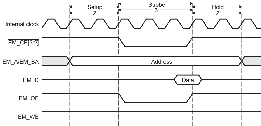
Figure 6. Timing Waveform of an Asynchronous Read Cycle in Select Strobe Mode
