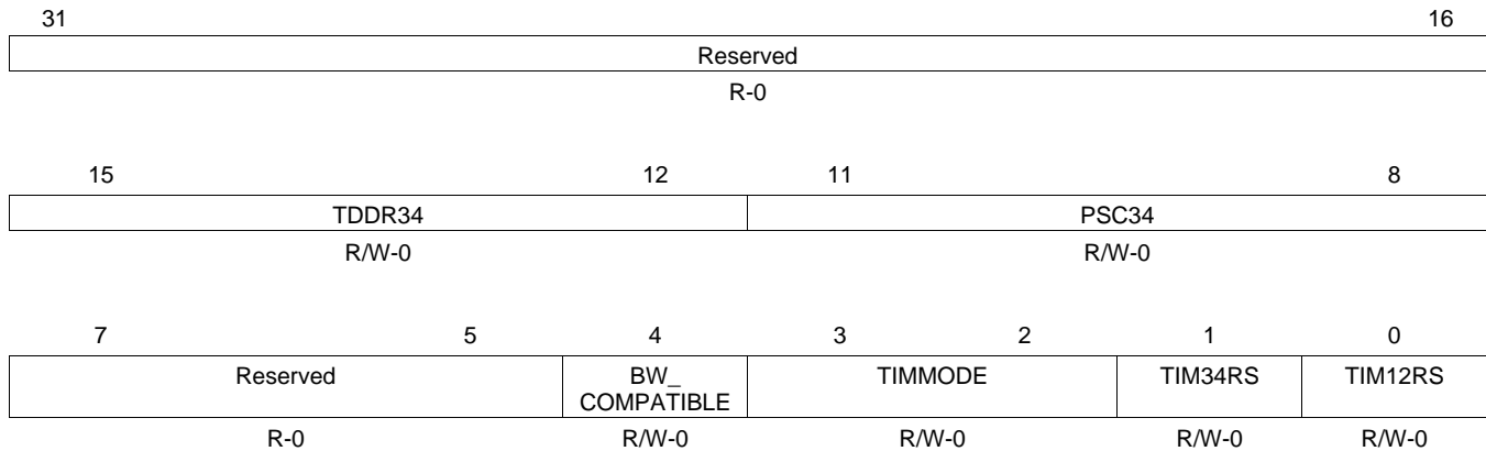
Figure 19. Timer Global Control Register (TGCR)
