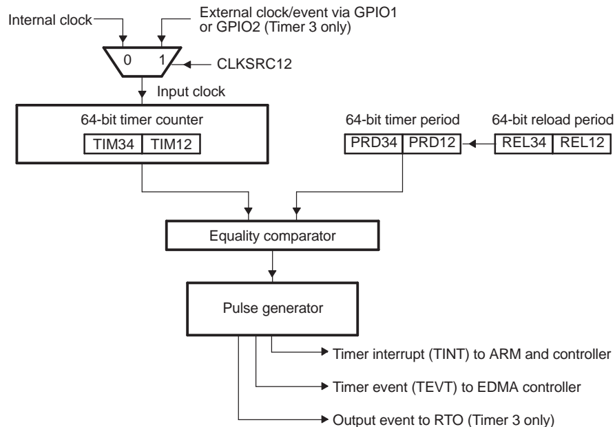
Figure 3. 64-Bit Timer Mode Block Diagram
