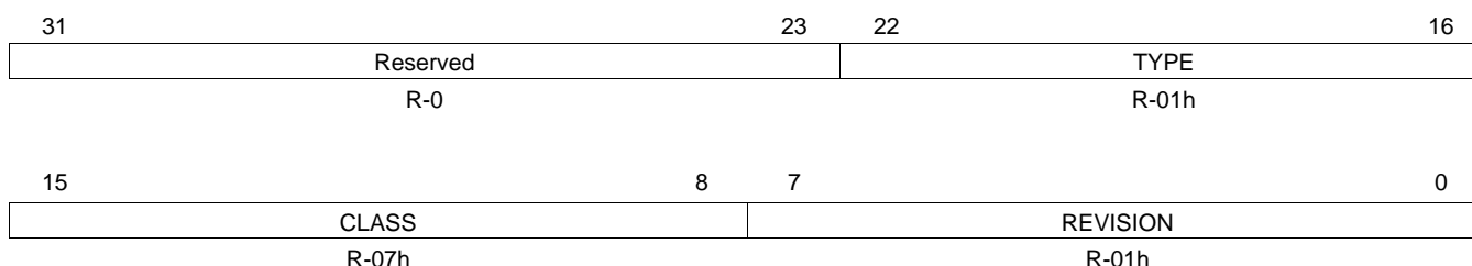
Figure 11. Timer 0, Timer 1, and Timer 2 Peripheral Identification Register 12 (PID12)
