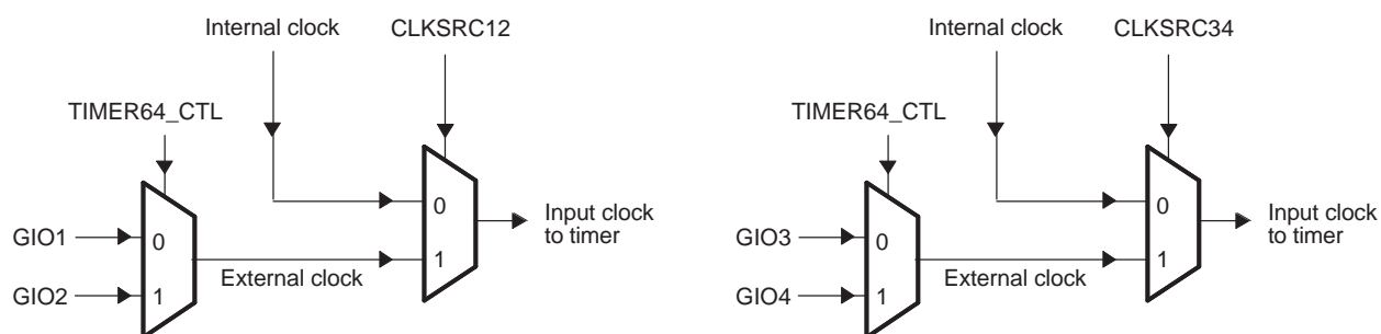
Figure 2. Timer Clock Source Block Diagram
