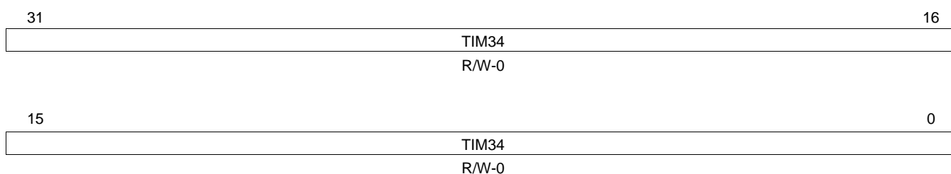
Figure 15. Timer Counter Register 34 (TIM34)
