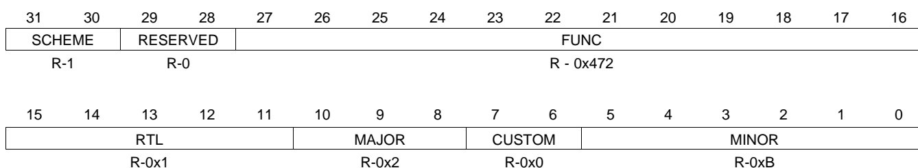
Figure 12. Timer 3 Peripheral Identification Register 12 (PID12)
