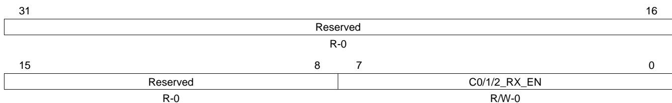
Figure 19. Core 0/1/2 Receive Enable Register (C0/1/2_RX_EN)
