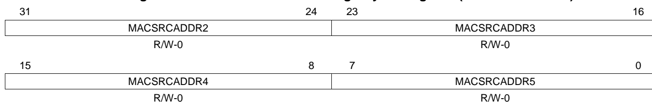
Figure 72. MAC Source Address High Bytes Register (MACSRCADDRHI)
