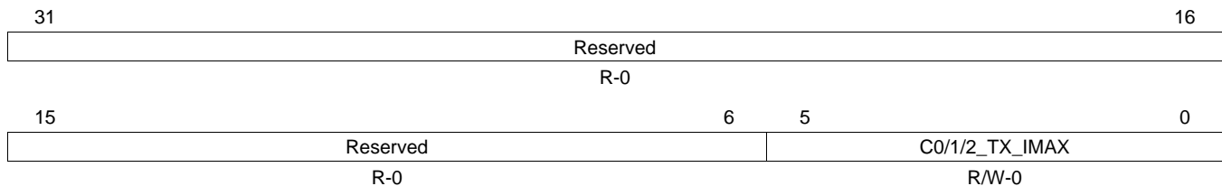
Figure 27. Core 0/1/2 Transmit Interrupts per Millisecond Register (C0/1/2_TX_IMAX)
