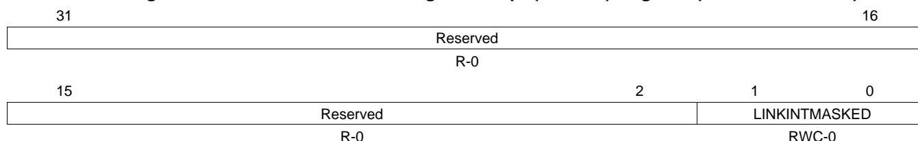
Figure 92. MDIO Link Status Change Interrupt (Masked) Register (LINKINTMASKED)
