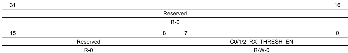
Figure 18. Core 0/1/2 Receive Threshold Enable Register (C0/1/2_RX_THRESH_EN)
