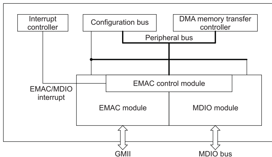
Figure 1. EMAC and MDIO Block Diagram
