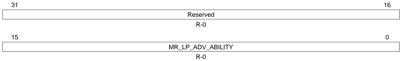
Figure 33. Link Partner Advertised Ability Register MR_LP_ADV_ABILITY (Mr_Lp_Adv_Ability)
