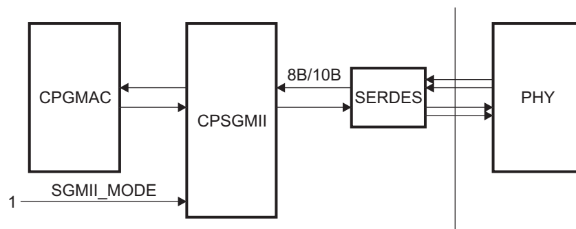
Figure 11. CPGMAC to PHY Interface
