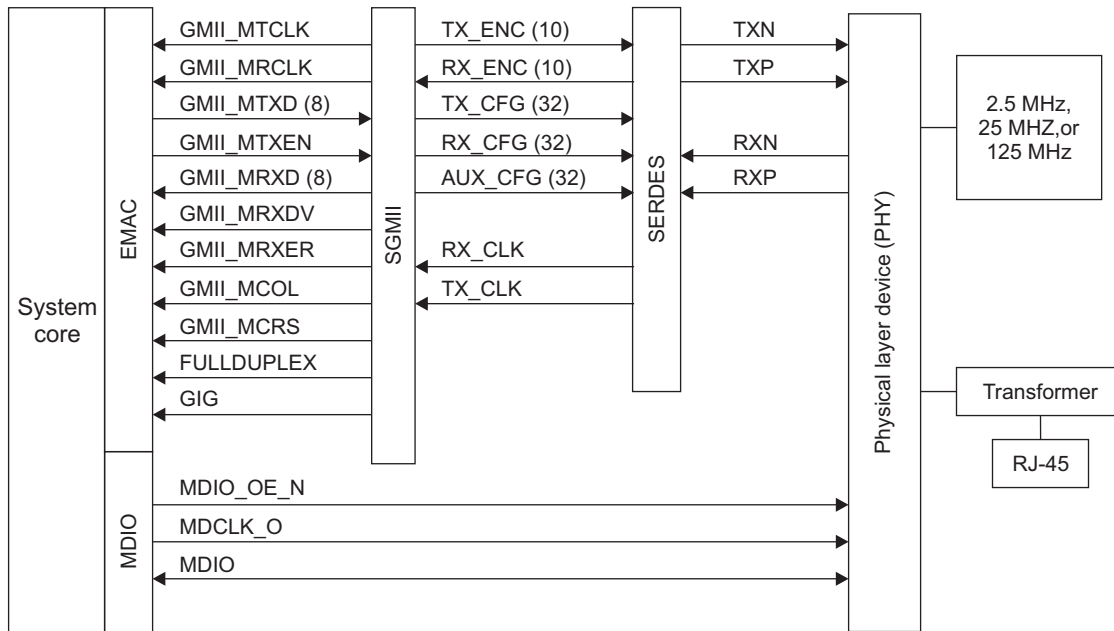
Figure 2. Ethernet Configuration with SGMII Interface
