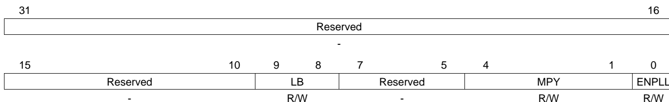
Figure 36. Auxiliary Configuration Register (AUX_CFG)
