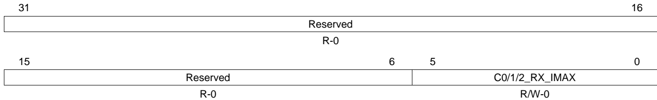
Figure 26. Core 0/1/2 Receive Interrupts per Millisecond Register (C0/1/2_RX_IMAX)
