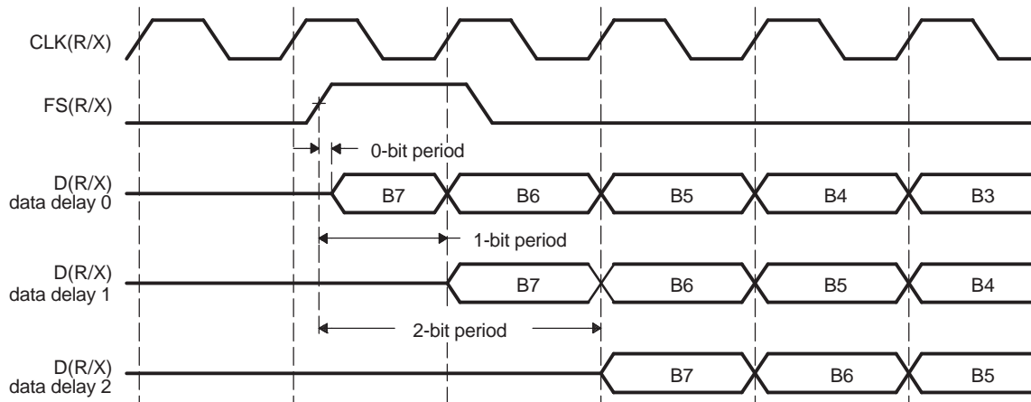
Figure 13. Data Delay
