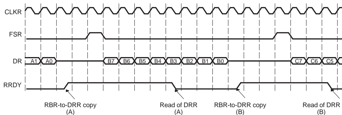
Figure 22. Receive Operation
