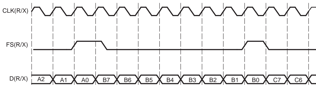
Figure 24. Maximum Frame Frequency for Transmit and Receive
