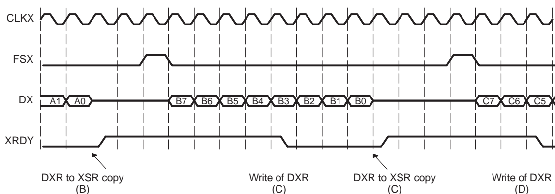
Figure 23. Transmit Operation
