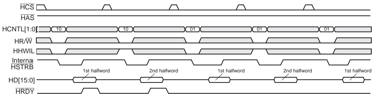
Figure 12. \overline{\text{HRDY}} Behavior During a Data Write Operation in the Multiplexed Mode (Case 2: Autoincrementing Selected, FIFO Empty Before Write)
