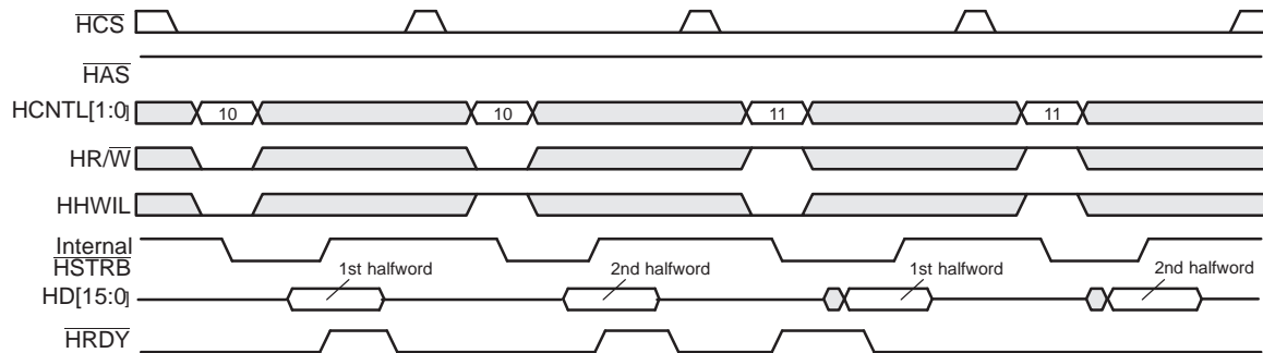
Figure 8. HRDY Behavior During a Data Read Operation in the Multiplexed Mode (Case 1: HPIA Write Cycle Followed by Nonautoincrement HPID Read Cycle)
