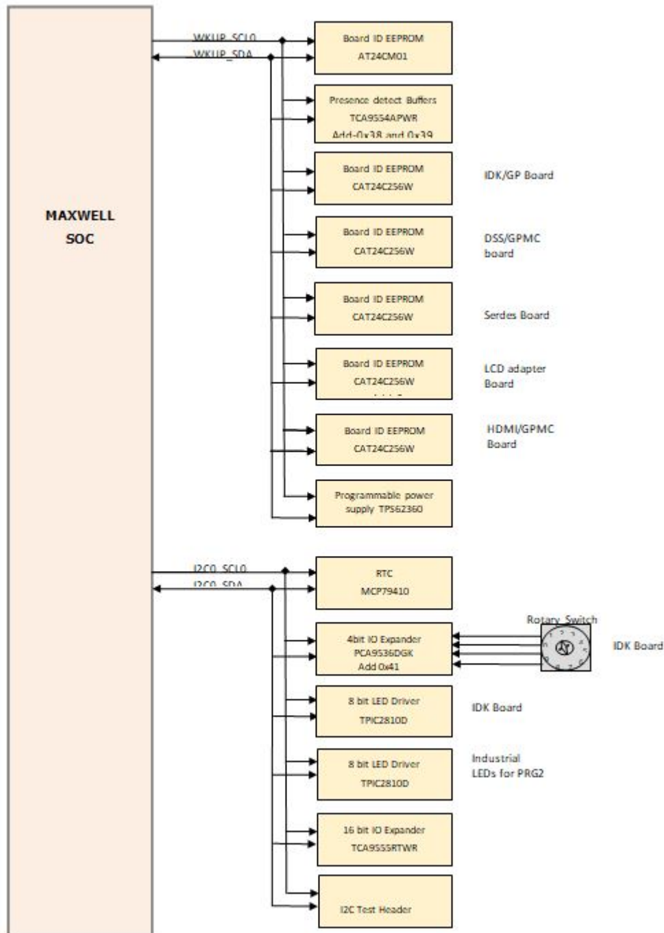
Figure 24. I2C Interfaces and Address Assignment to its Peripherals (1 of 2)
