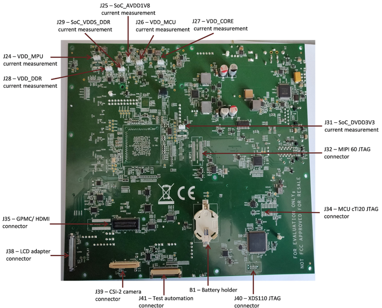
Figure 4. Bottom View of the Common Processor Board
