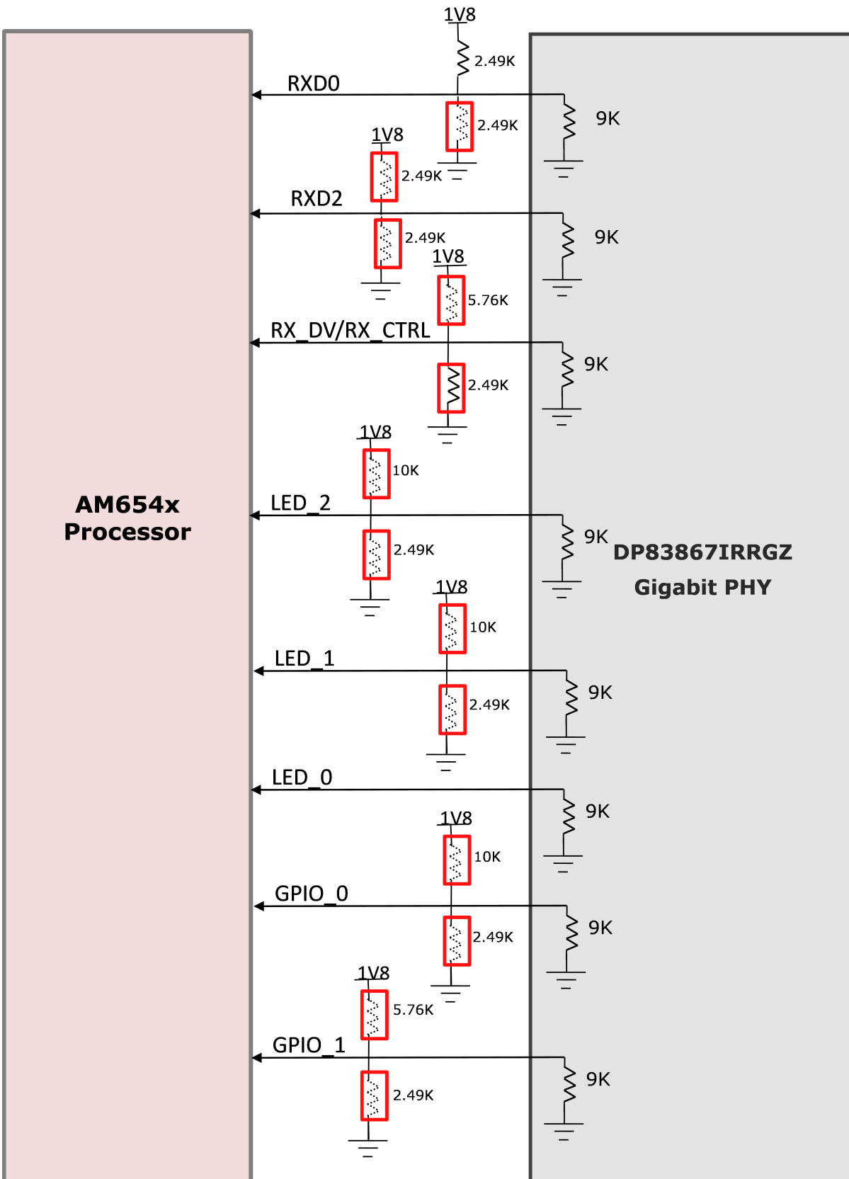
Figure 19. Strapping Diagram for PRG2-RGMII2 Ethernet
