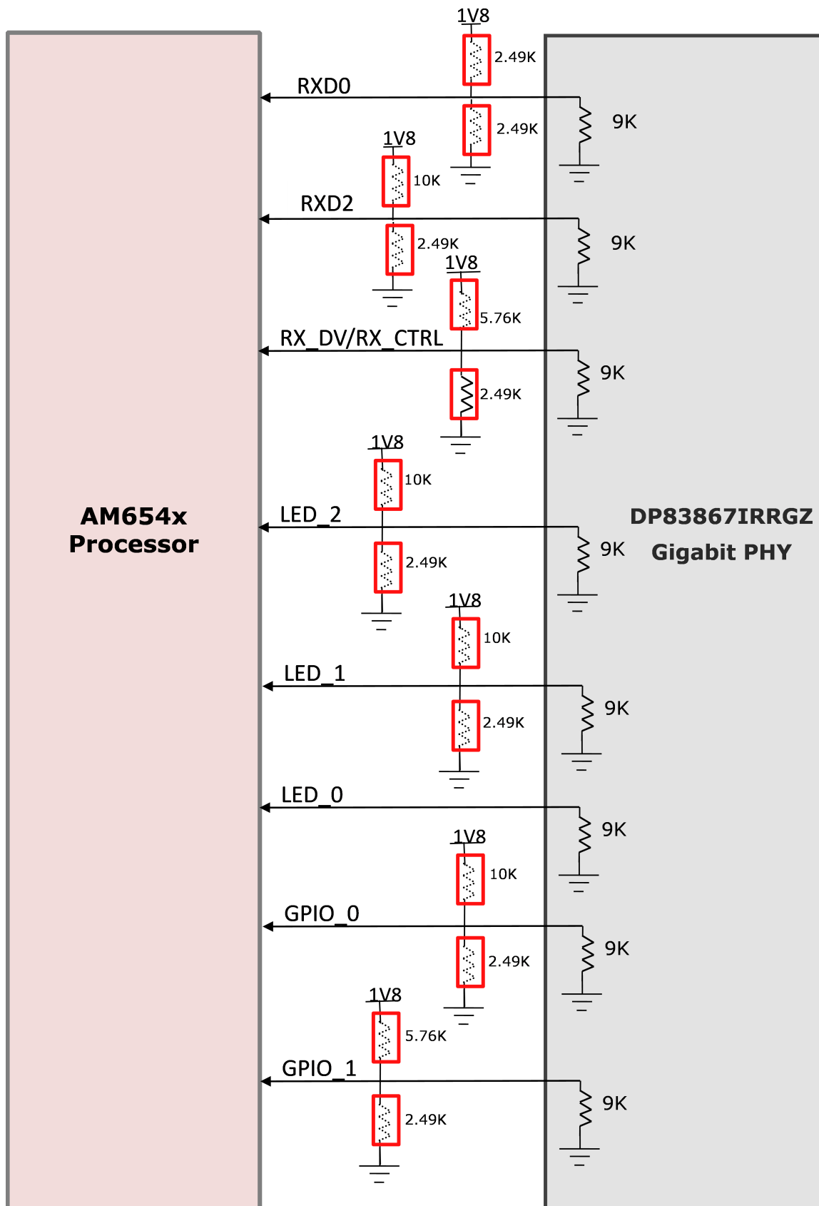
Figure 18. Strapping Diagram for MCU and PRG2-RGMII1 Ethernet
