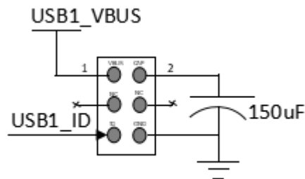
Figure 21. J4 Header for USB2.0 Host Interface
