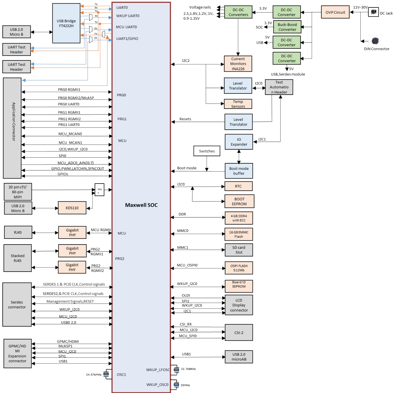
Figure 5. Common Processor Board Functional Block Diagram
