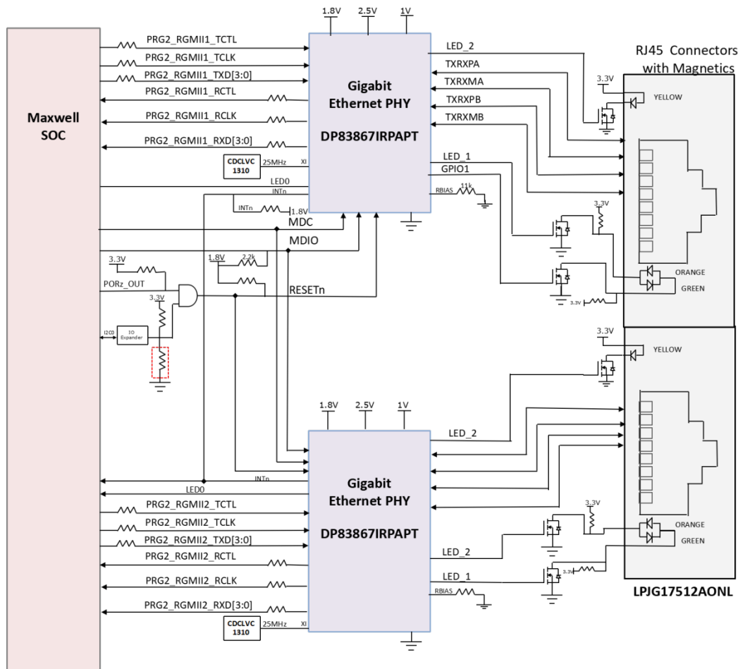
Figure 17. Ethernet Interface – ICSSG Domain
