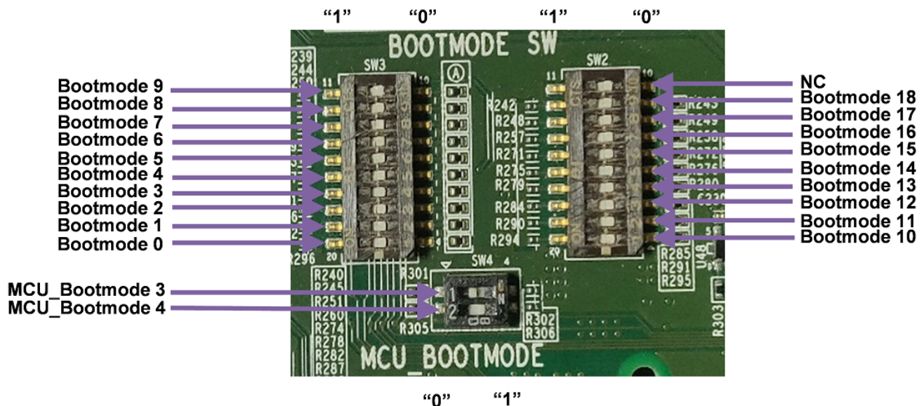
Figure 11. BOOT Switches Provided on the Processor Card
