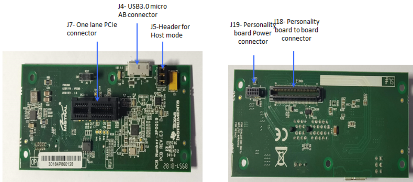
Figure 29. x2 Lane PCIe Card
