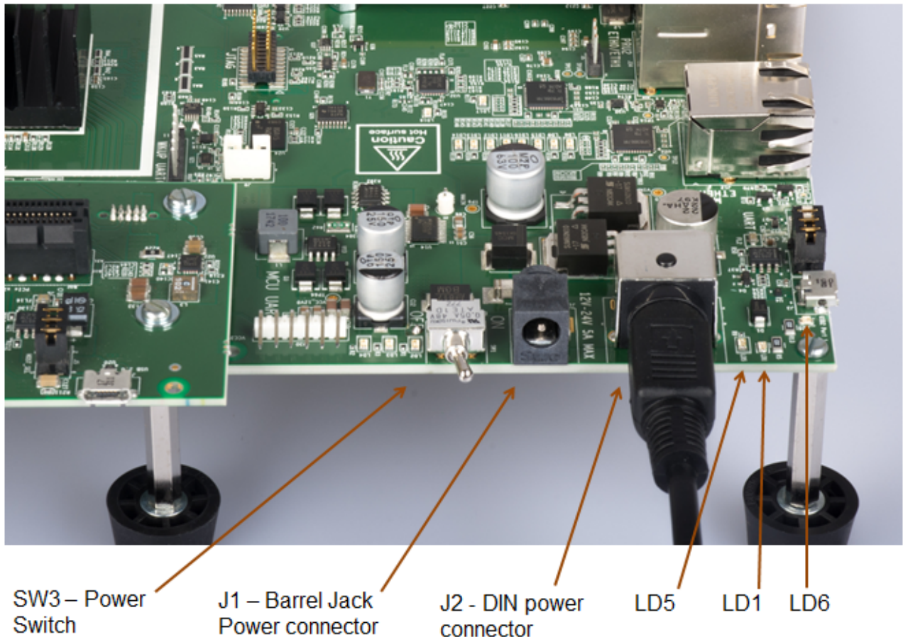
Figure 8. Connectors Used for Power Input
