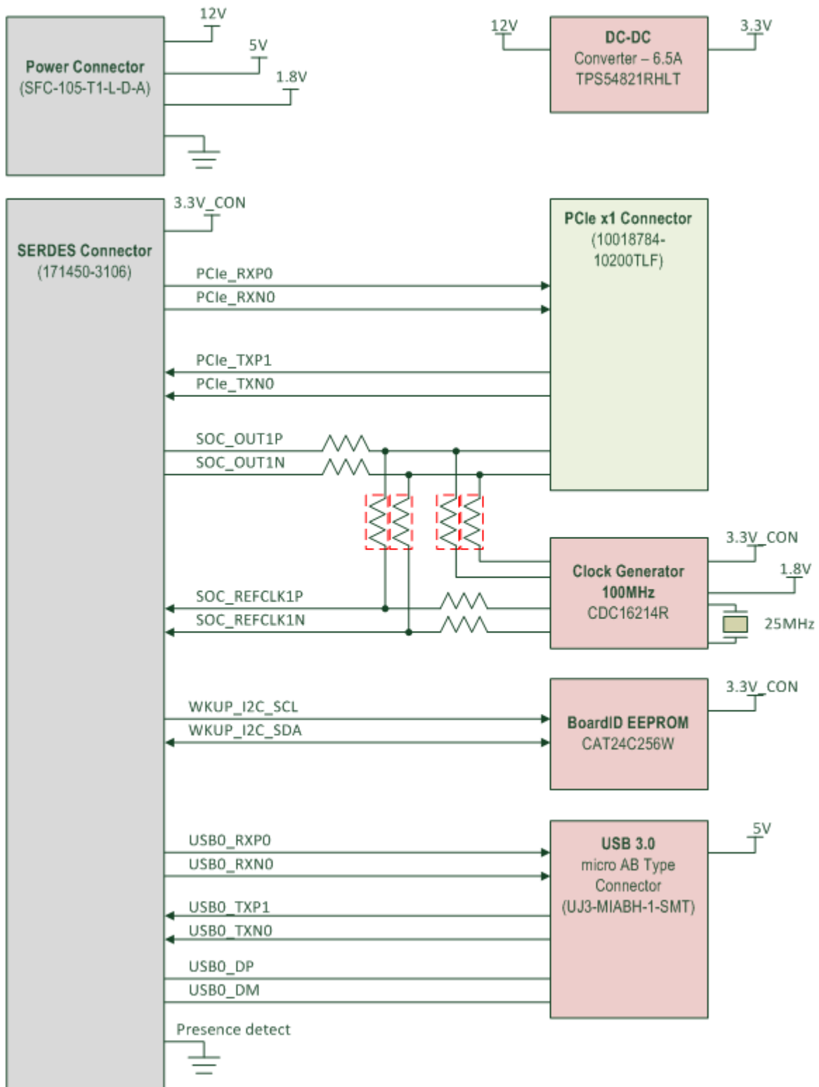
Figure 30. x1 Lane PCIe/USB3 Personality Card Block Diagram
