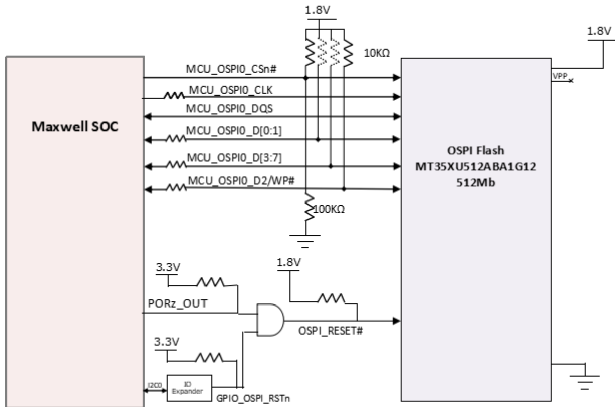
Figure 15. OSPI Interface
