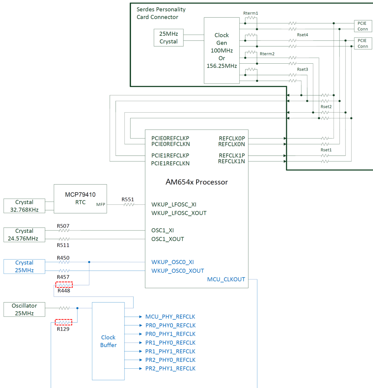
Figure 6. AM65x GP EVM Clock Tree
