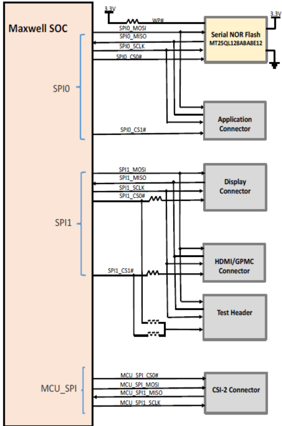
Figure 26. SPI Tree
