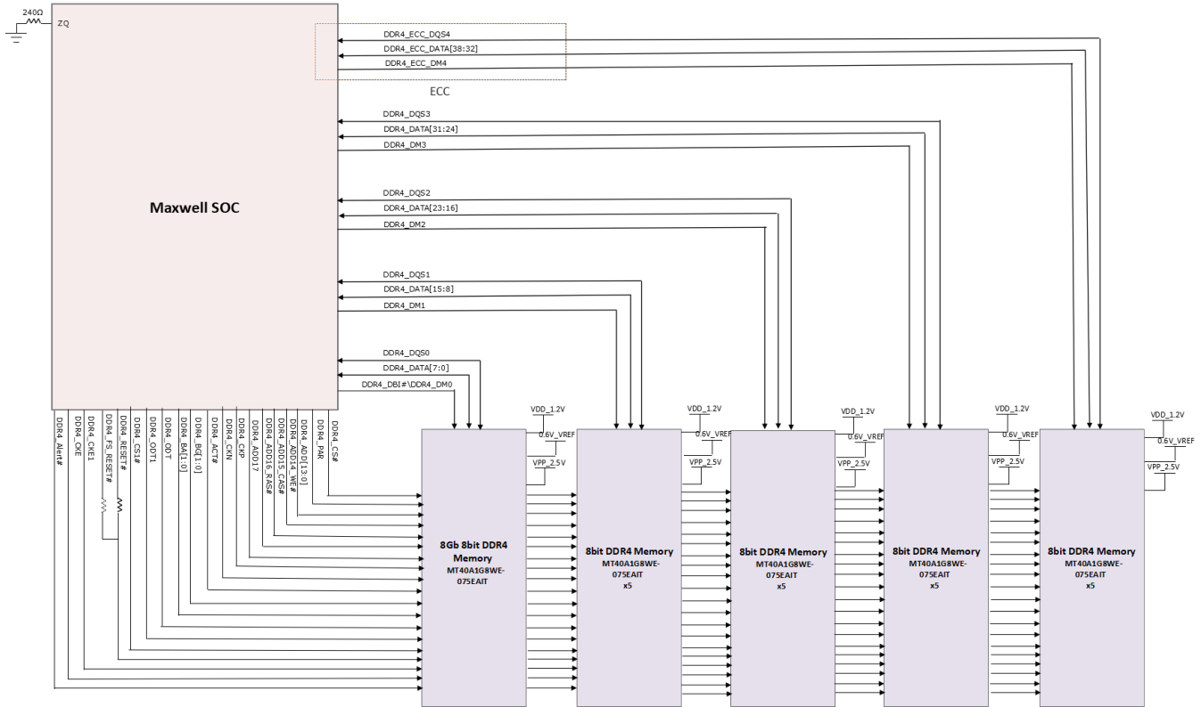
Figure 12. DDR4 Interface
