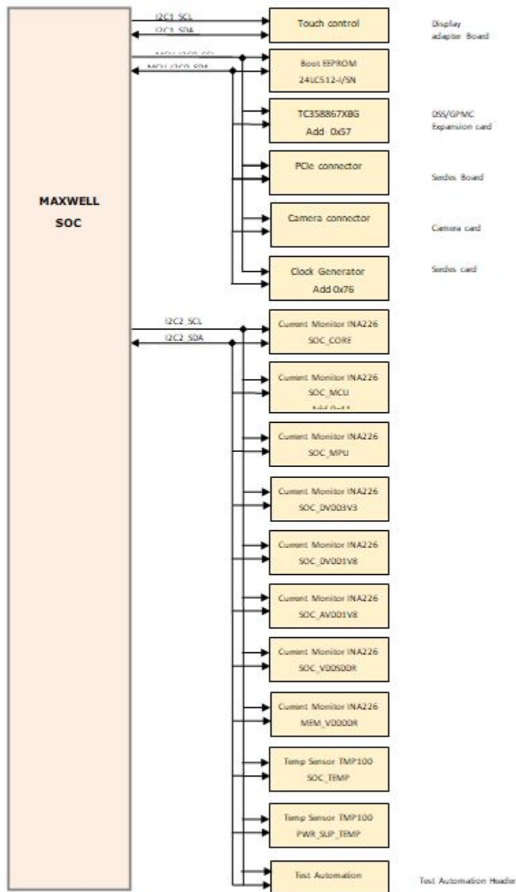
Figure 25. I2C Interfaces and Address Assignment to its Peripherals (2 of 2)
