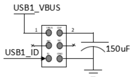
Figure 31. J5 Header for USB 3.0 Host Operation
