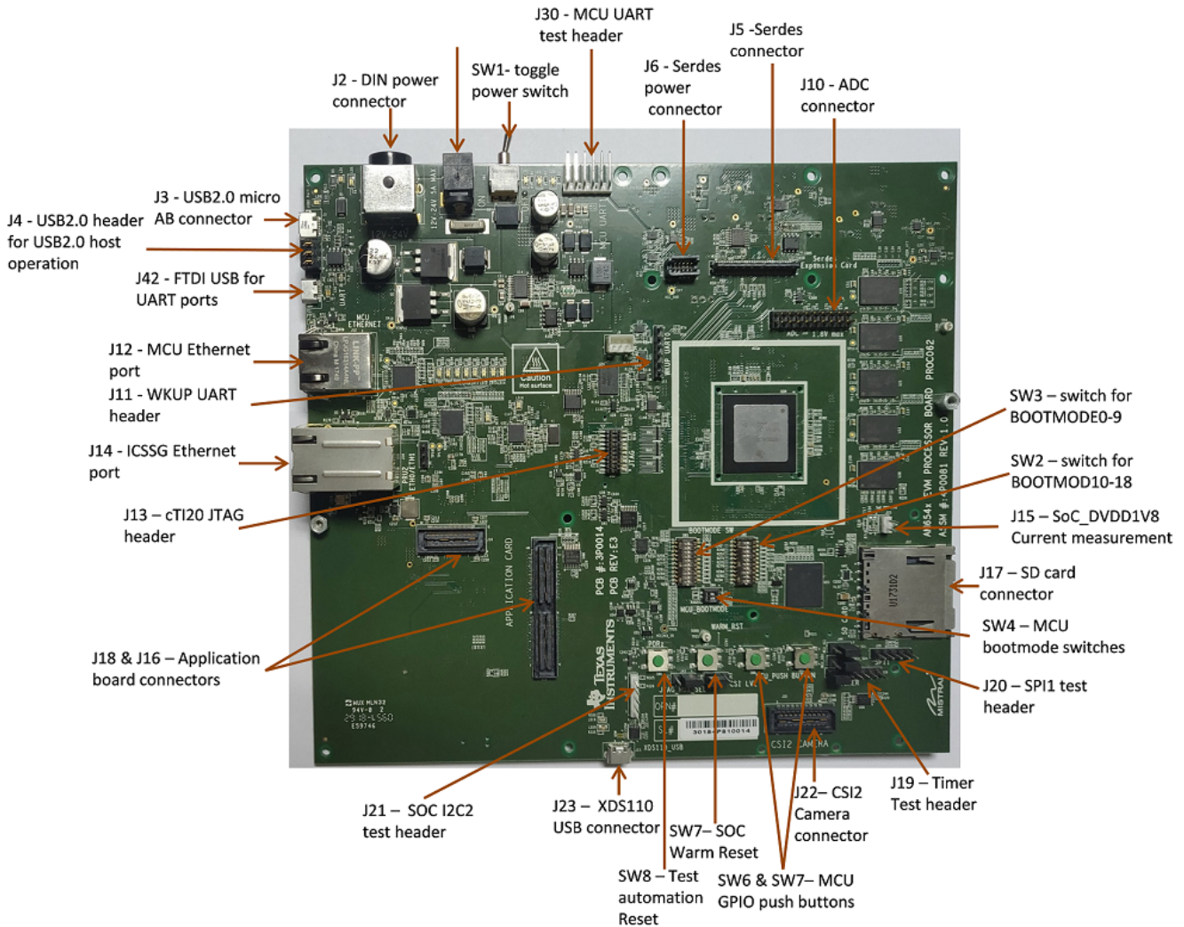
Figure 3. Top View of the Common Processor Board
