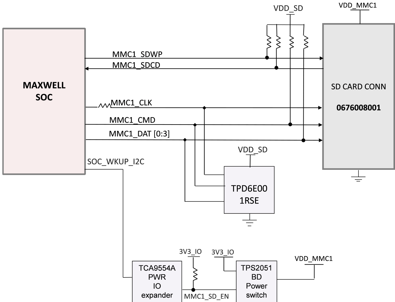
Figure 13. SDHC Interface
