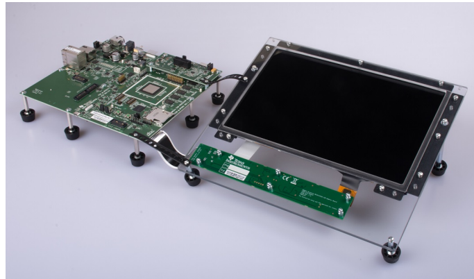
Figure 1. System Assembly Image
