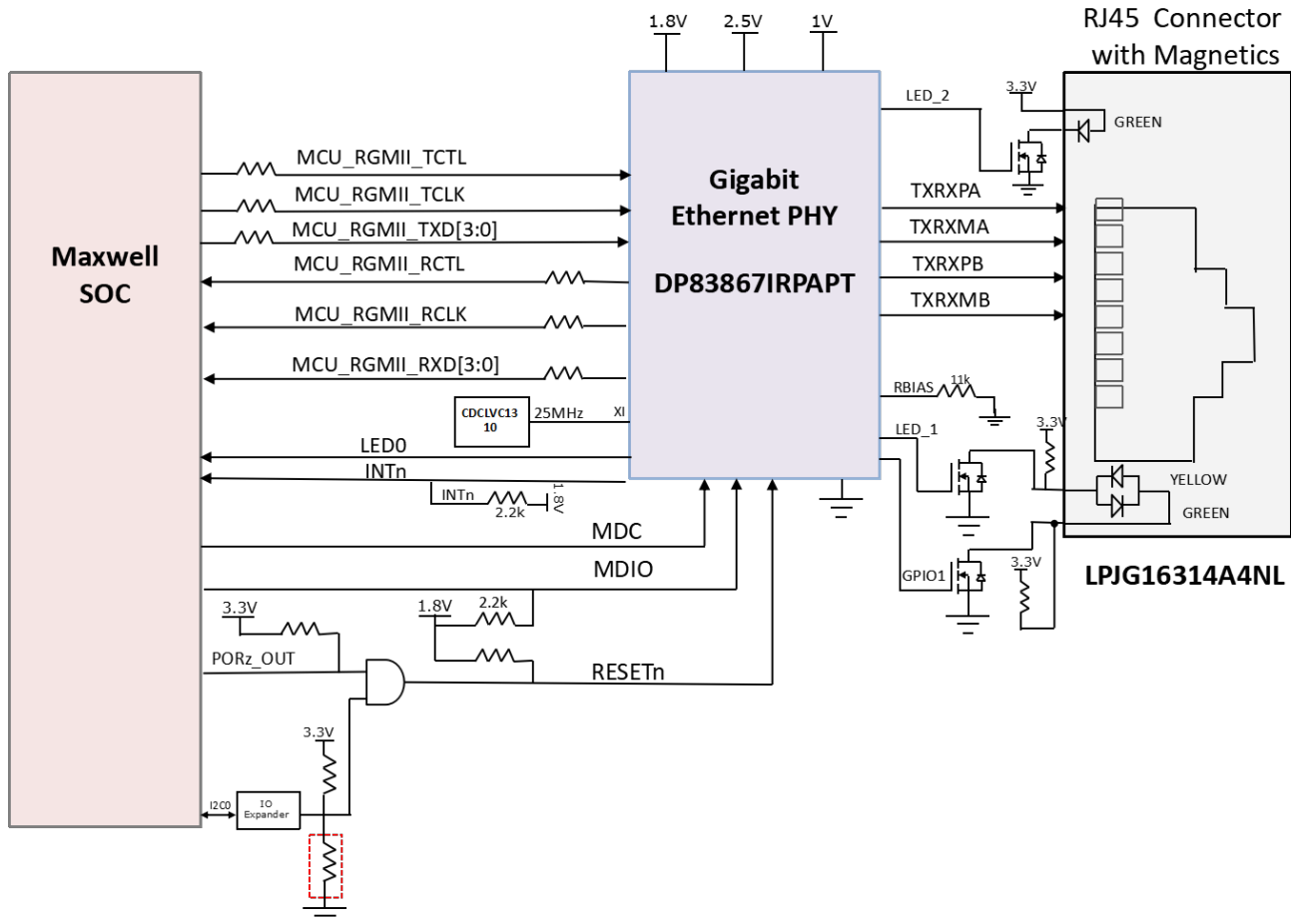
Figure 16. Ethernet Interface – MCU Domain
