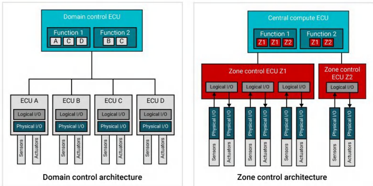
Figure 5. Separation of logical and physical I/O functionality from a domain architecture to a zone architecture.
