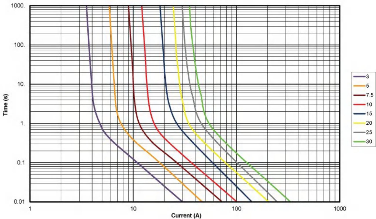
Figure 4. TCC curves of Littelfuse microfuses.
