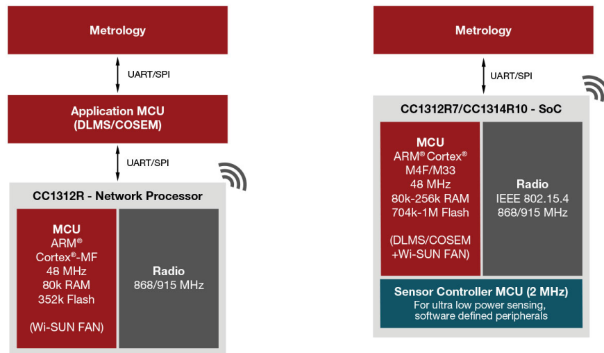
Figure 1. Architecture Options for a Smart-Meter Router Node
