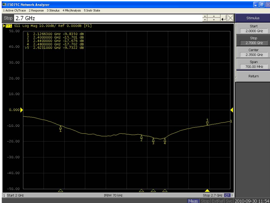
Figure 7. Bandwidth Measurement
