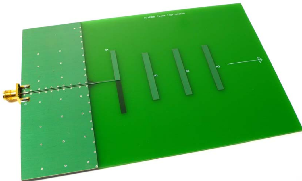
Figure 1. 2.4 GHz Yagi PCB Directional Antenna Test Board
