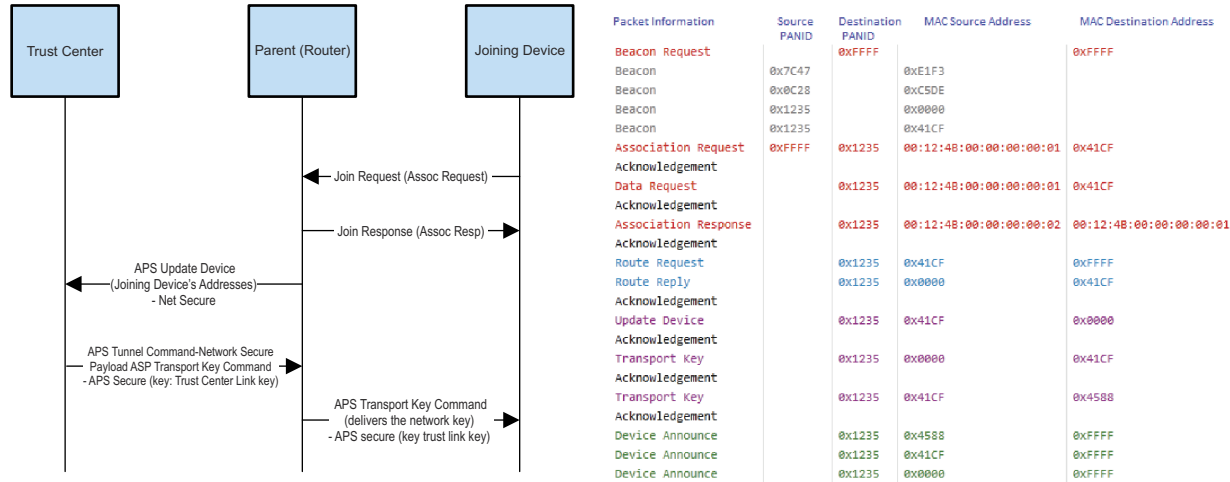
Figure 2-3. (a) Network Join Sequence When the Parent is not the Trust Center (b) Ubiqua Log Snapshot Showing Over the Air Messages During Network Join Procedure
