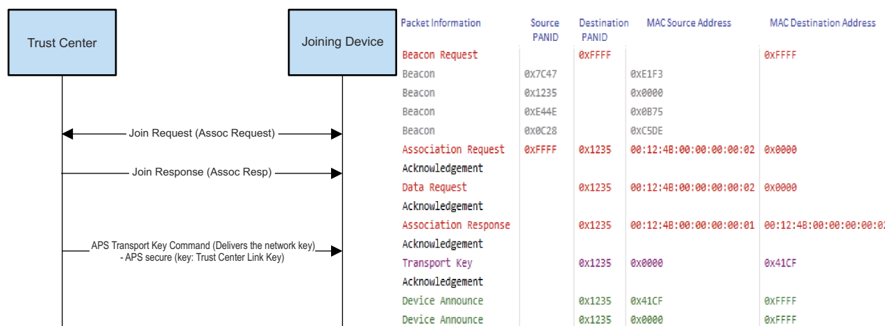
Figure 2-2. (a) Network Join Sequence When the Parent is the Trust Center (b) Ubiqua Log Snapshot Showing Over the Air Messages During Network Join Procedure
