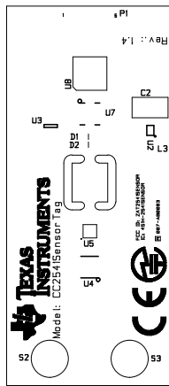
SILK SCREEN PRIMARY SIDE VIEWED FROM PRIMARY SIDE
