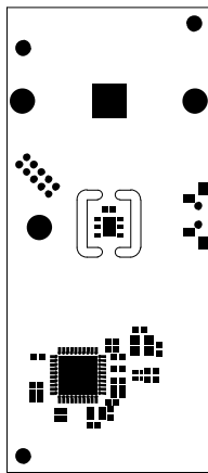
SOLDER RESIST SECONDARY SIDE VIEWED FROM PRIMARY SIDE
