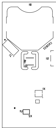
SILK SCREEN SECONDARY SIDE VIEWED FROM PRIMARY SIDE
