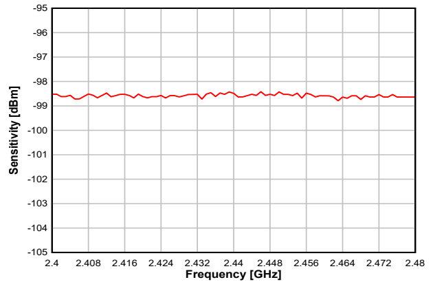
Figure 8-11. Sensitivity vs. Frequency (IEEE 802.15.4-2006, 250 kbps, OQPSK DSSS 1:8, 2.44 GHz)
