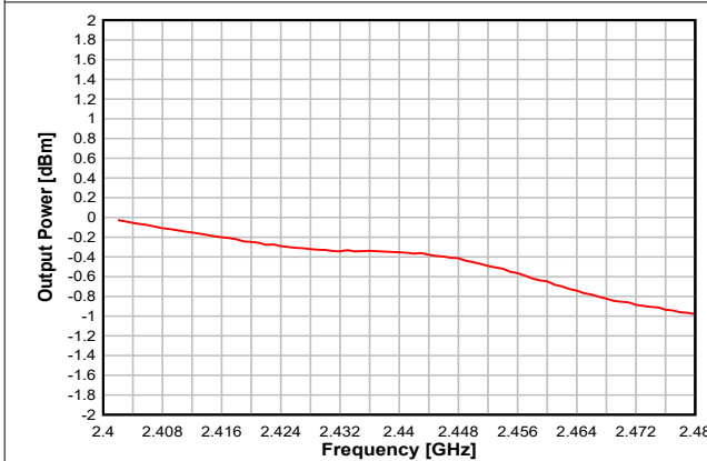
Figure 8-21. Output Power vs. Frequency (BLE 1 Mbps, 2.44 GHz, 0 dBm)
