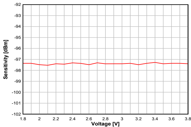
Figure 8-14. Sensitivity vs. Supply Voltage (VDDS) (BLE 1 Mbps, 2.44 GHz)
