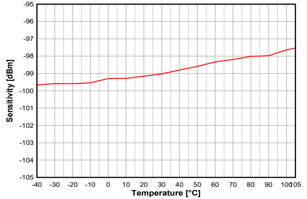
Figure 8-13. Sensitivity vs. Temperature (IEEE 802.15.4-2006, 250 kbps, OQPSK DSSS 1:8, 2.44 GHz)
