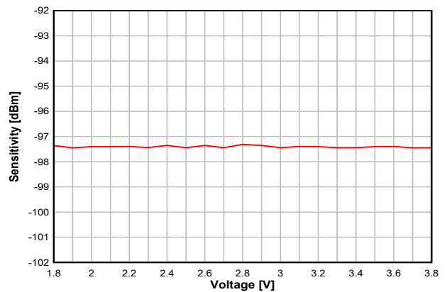
Figure 8-15. Sensitivity vs. Supply Voltage (VDDS) (BLE 1 Mbps, 2.44 GHz, DCDC Off)
