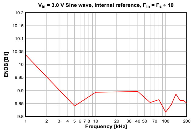
Figure 7-36. ENOB vs. Sampling Frequency
