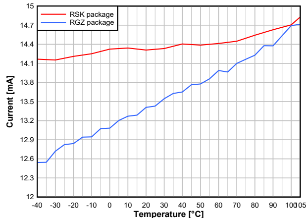
Figure 7-10. TX Current vs. Temperature (50kbps, 868.3MHz, +10dBm, VDD = 3.6V)
