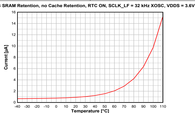
Figure 7-5. Standby Mode (MCU) Current vs. Temperature (VDD5 = 3.6V)
