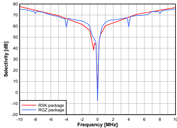
Figure 7-24. Selectivity vs. Frequency Offset (50kbps, 868.3MHz)
