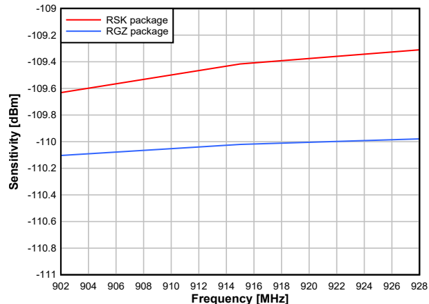
Figure 7-15. Sensitivity vs. Frequency (50kbps, 915MHz)
