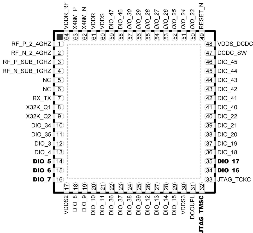
Figure 6-2. RSK (8mm × 8mm) Pinout, 0.4mm Pitch (Top View)
