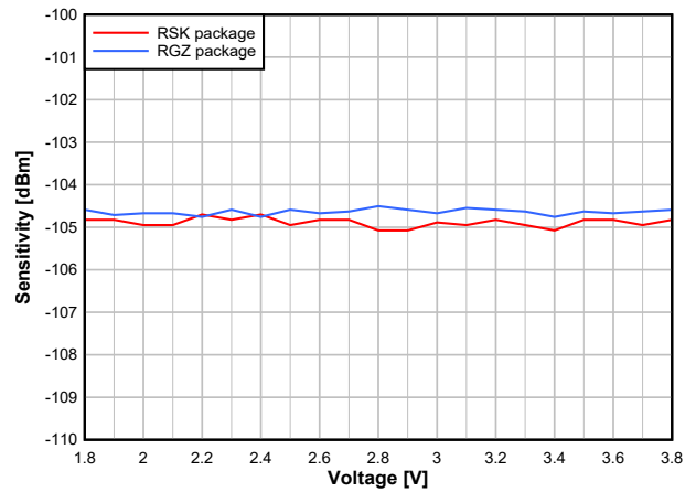
Figure 7-23. Sensitivity vs. Supply Voltage (VDD) (250kbps, 2.44GHz)
