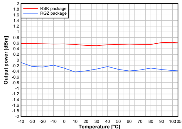
Figure 7-26. Output Power vs. Temperature (BLE 1Mbps, 2.44GHz, 0dBm)
