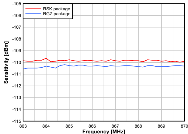
Figure 7-14. Sensitivity vs. Frequency (50kbps, 868MHz)
