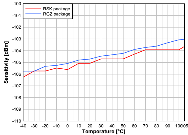
Figure 7-20. Sensitivity vs. Temperature (250kbps, 2.44GHz)
