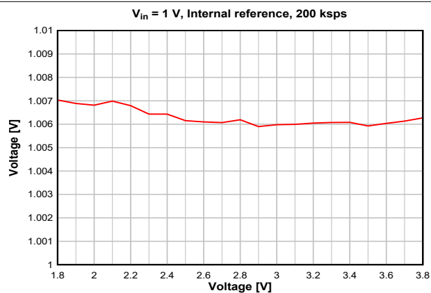
Figure 7-40. ADC Accuracy vs. Supply Voltage (VDD)
