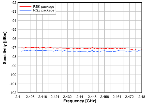
Figure 7-16. Sensitivity vs. Frequency (BLE 1Mbps, 2.44GHz)
