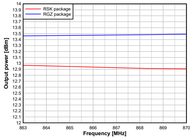
Figure 7-31. Output Power vs. Frequency (50kbps, 868MHz, +14dBm)
