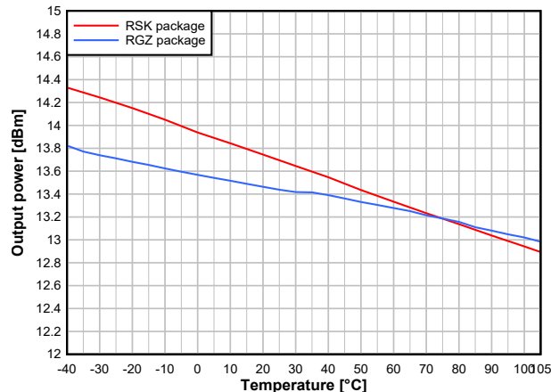
Figure 7-25. Output Power vs. Temperature (50kbps, 868.3MHz, +14dBm)
