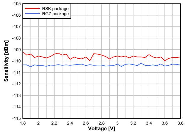
Figure 7-21. Sensitivity vs. Supply Voltage (VDD) (50kbps, 868.3MHz)
