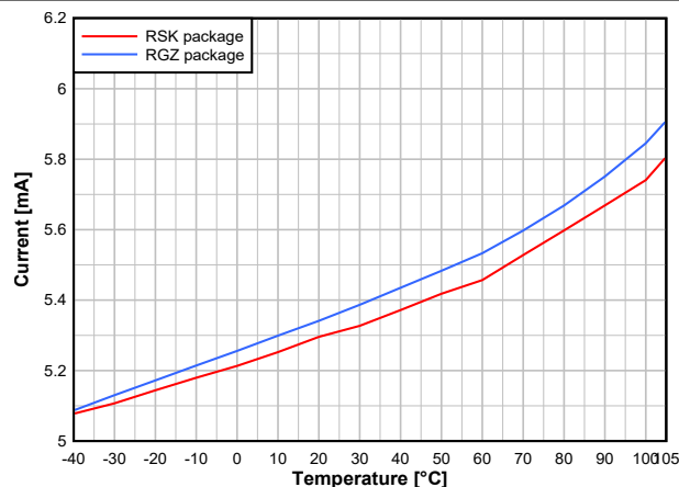
Figure 7-6. RX Current vs. Temperature (50kbps, 868.3MHz, VDD5 = 3.6V)
