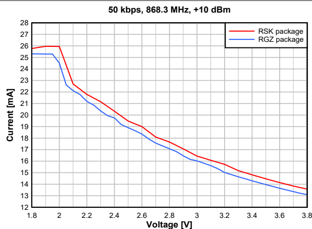
Figure 7-12. TX Current vs. Supply Voltage (VDD) (50kbps, 868.3MHz)
