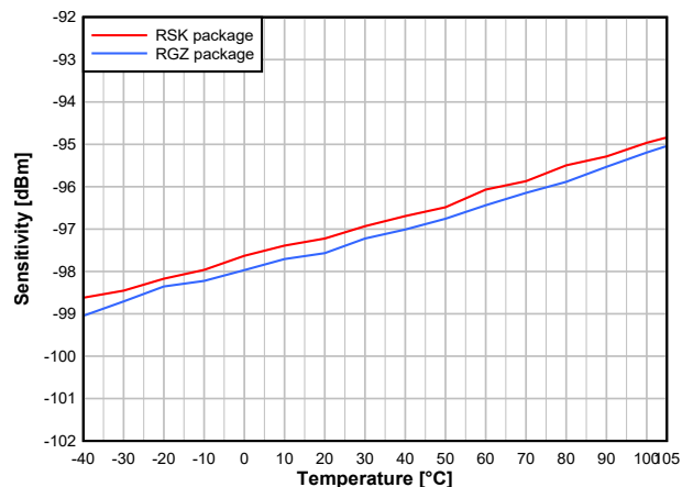
Figure 7-19. Sensitivity vs. Temperature (BLE 1 Mbps, 2.44GHz)
