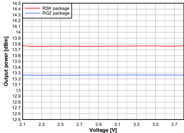
Figure 7-28. Output Power vs. Supply Voltage (VDDS) (50kbps, 868.3MHz, +14dBm)
