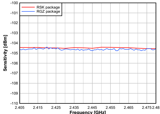
Figure 7-17. Sensitivity vs. Frequency (IEEE 802.15.4 OQPSK DSSS1:8, 250kbps, 2.44GHz)
