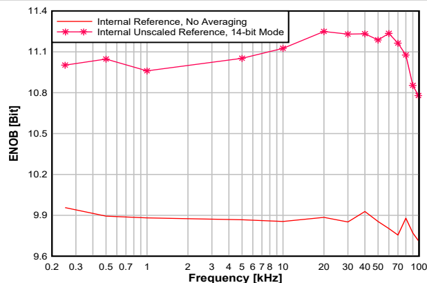
Figure 7-35. ENOB vs. Input Frequency
