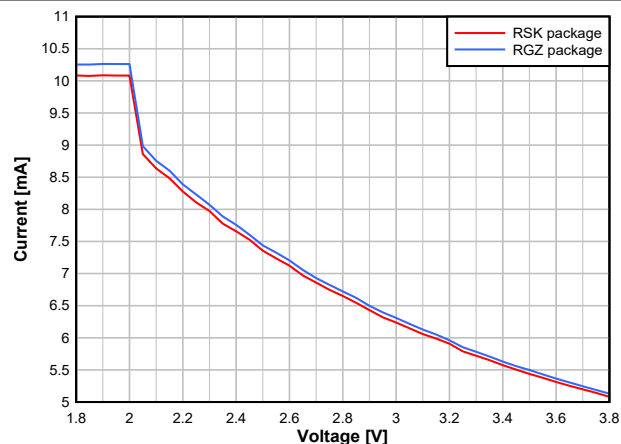
Figure 7-8. RX Current vs. Supply Voltage (VDD) (50kbps, 868.3MHz)
