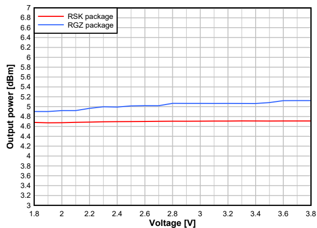
Figure 7-30. Output Power vs. Supply Voltage (VDDS) (BLE 1Mbps, 2.44GHz, +5dBm)
