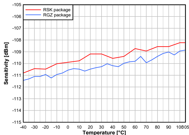
Figure 7-18. Sensitivity vs. Temperature (50kbps, 868.3MHz)
