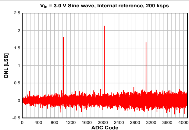
Figure 7-38. DNL vs. ADC Code
