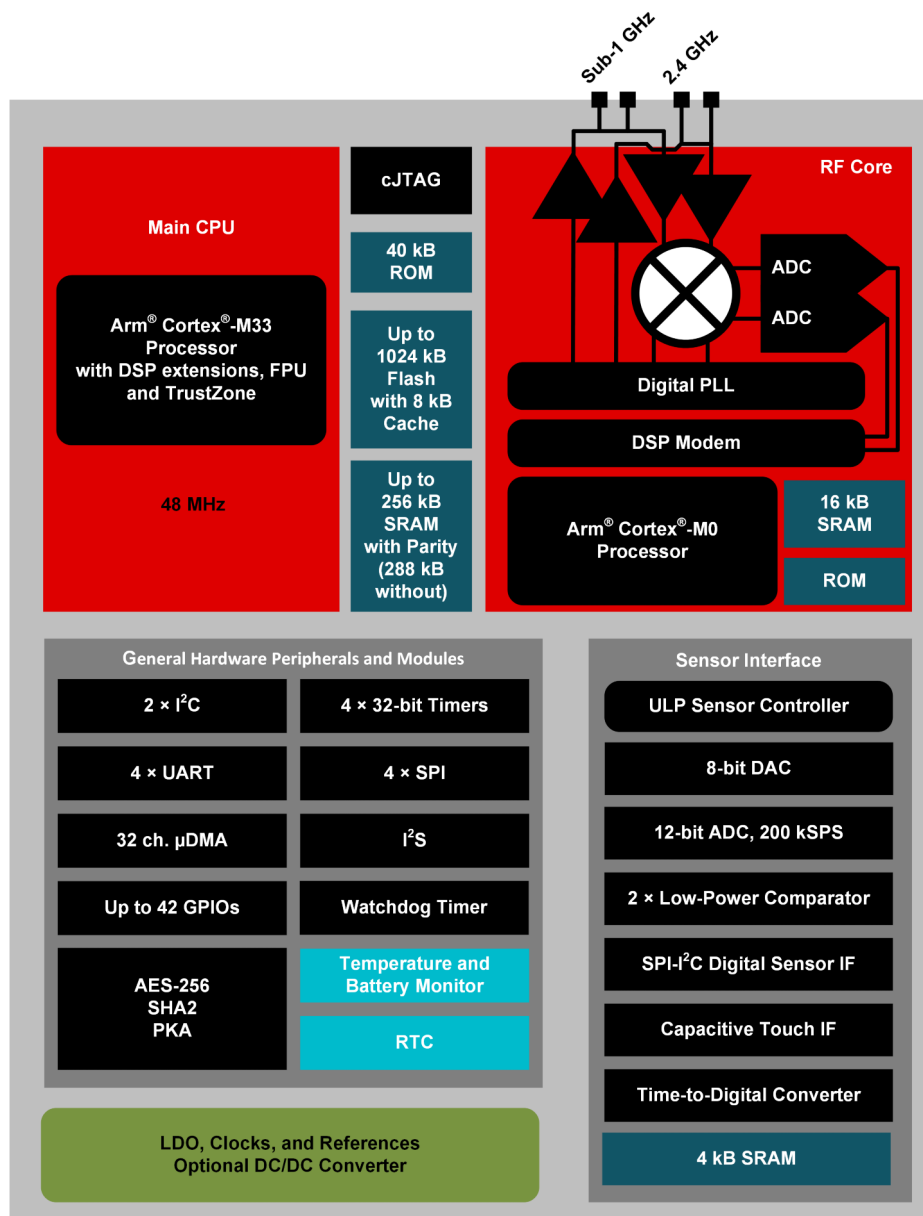
CC1354R10 Block Diagram
