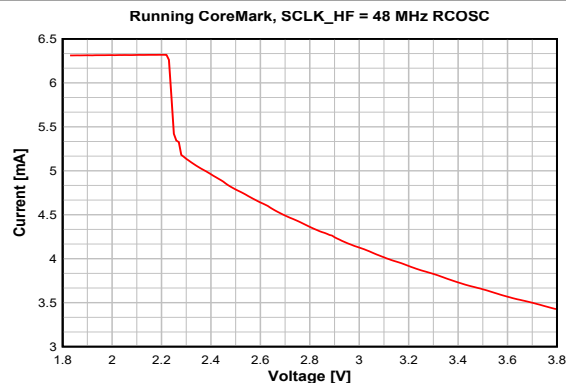
Figure 7-3. Active Mode (MCU) Current vs. Supply Voltage (VDD5)
