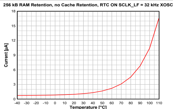
Figure 7-4. Standby Mode (MCU) Current vs. Temperature
