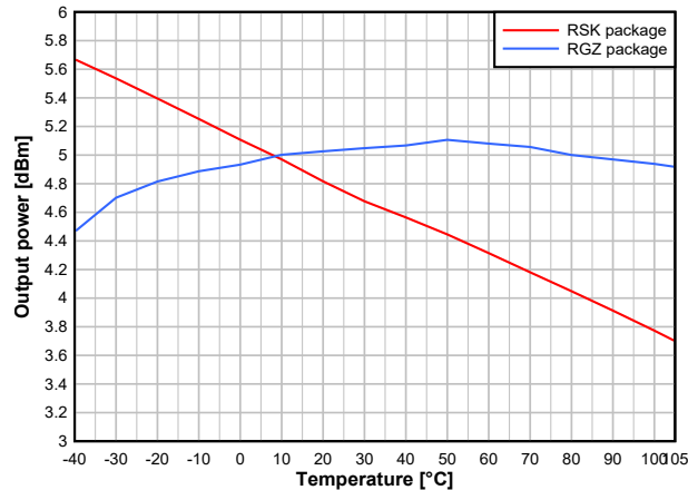
Figure 7-27. Output Power vs. Temperature (BLE 1Mbps, 2.44GHz, +5dBm)
