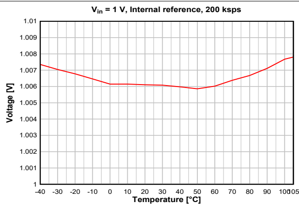
Figure 7-39. ADC Accuracy vs. Temperature
