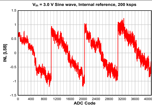
Figure 7-37. INL vs. ADC Code
