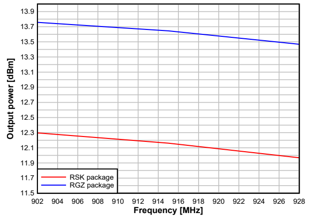
Figure 7-32. Output Power vs. Frequency (50kbps, 915MHz, +14dBm)
