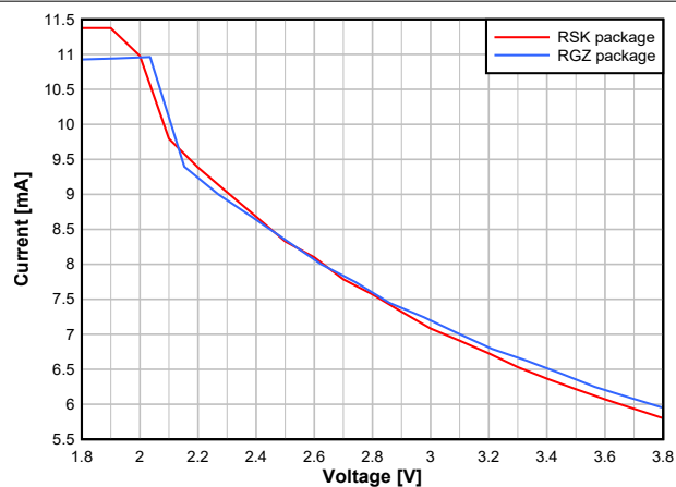
Figure 7-13. TX Current vs. Supply Voltage (VDD) (BLE 1 Mbps, 2.44GHz, 0dBm)
