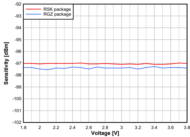
Figure 7-22. Sensitivity vs. Supply Voltage (VDD) (BLE 1Mbps, 2.44GHz)
