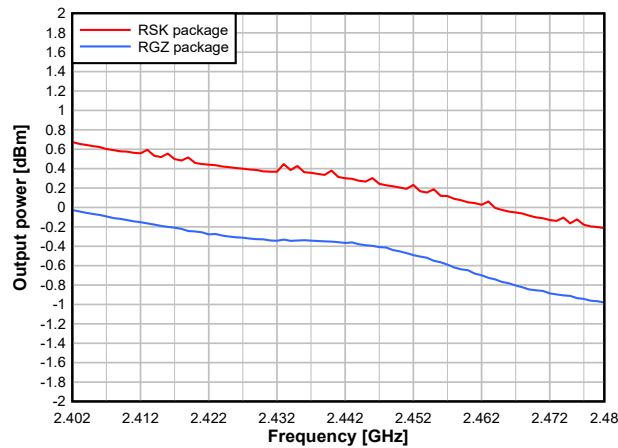
Figure 7-33. Output Power vs. Frequency (BLE 1Mbps, 2.44GHz, 0dBm)
