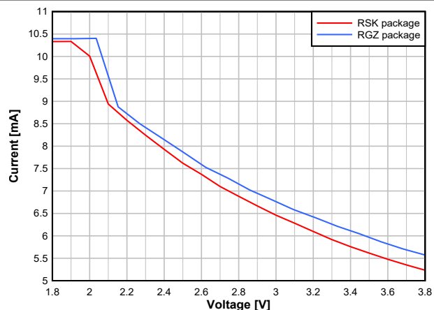
Figure 7-9. RX Current vs. Supply Voltage (VDD) (BLE 1Mbps, 2.44GHz)
