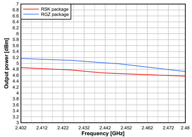
Figure 7-34. Output Power vs. Frequency (BLE 1Mbps, 2.44GHz, +5dBm)
