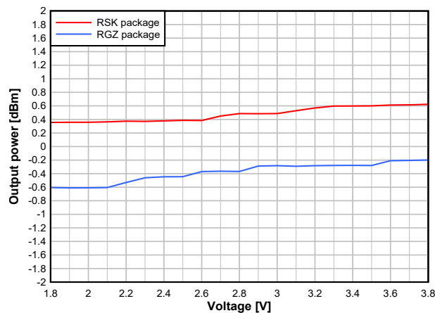
Figure 7-29. Output Power vs. Supply Voltage (VDDS) (BLE 1Mbps, 2.44GHz, 0dBm)
