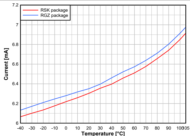
Figure 7-7. RX Current vs. Temperature (BLE 1Mbps, 2.44GHz)
