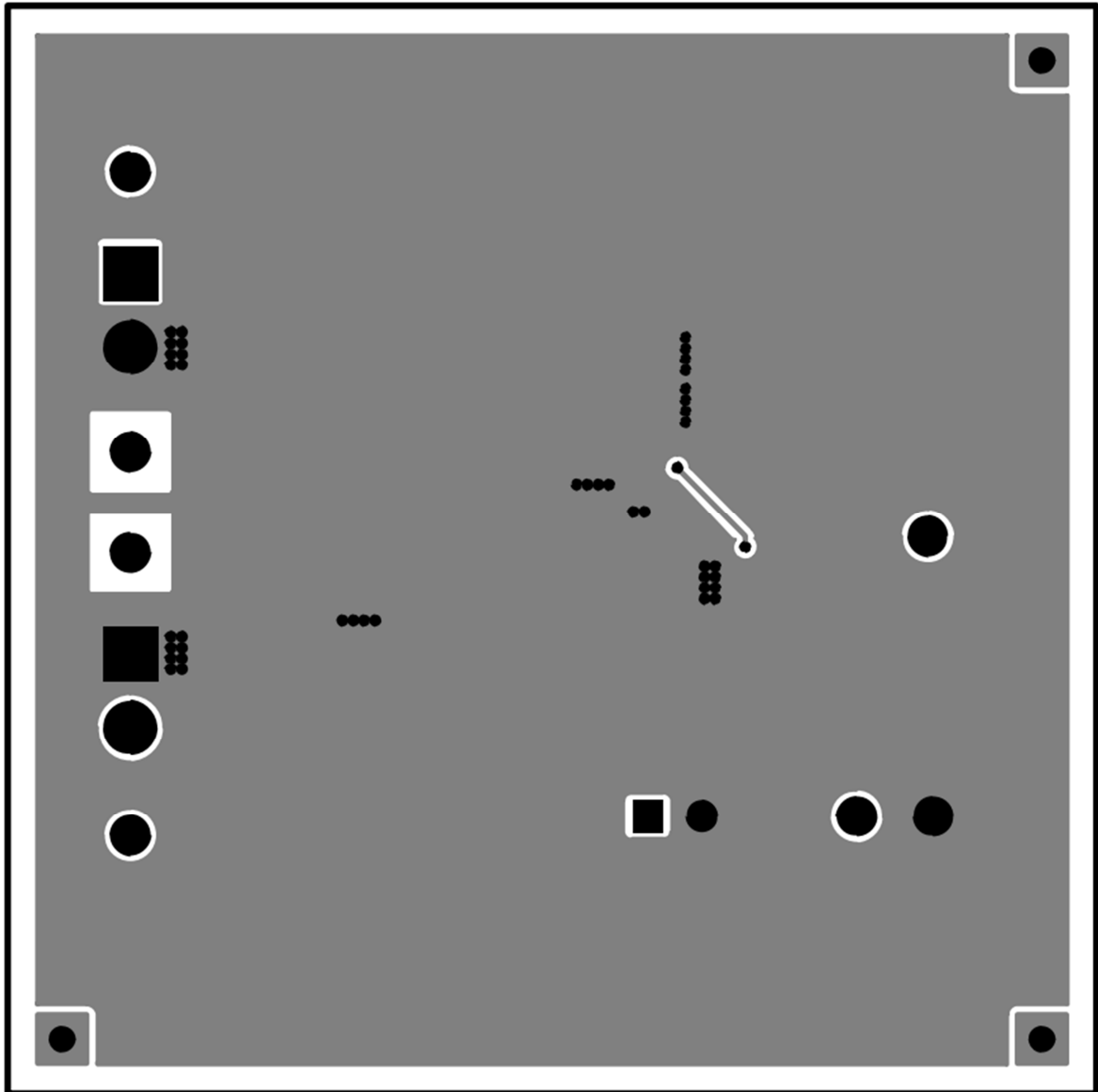
Figure 20. TPS54061EVM-142 Bottom-Side Assembly
