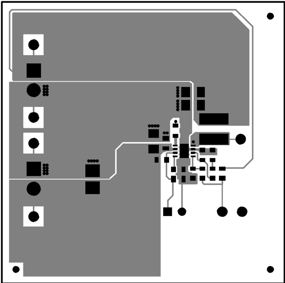
Figure 19. TPS54061EVM-142 Top-Side Layout
