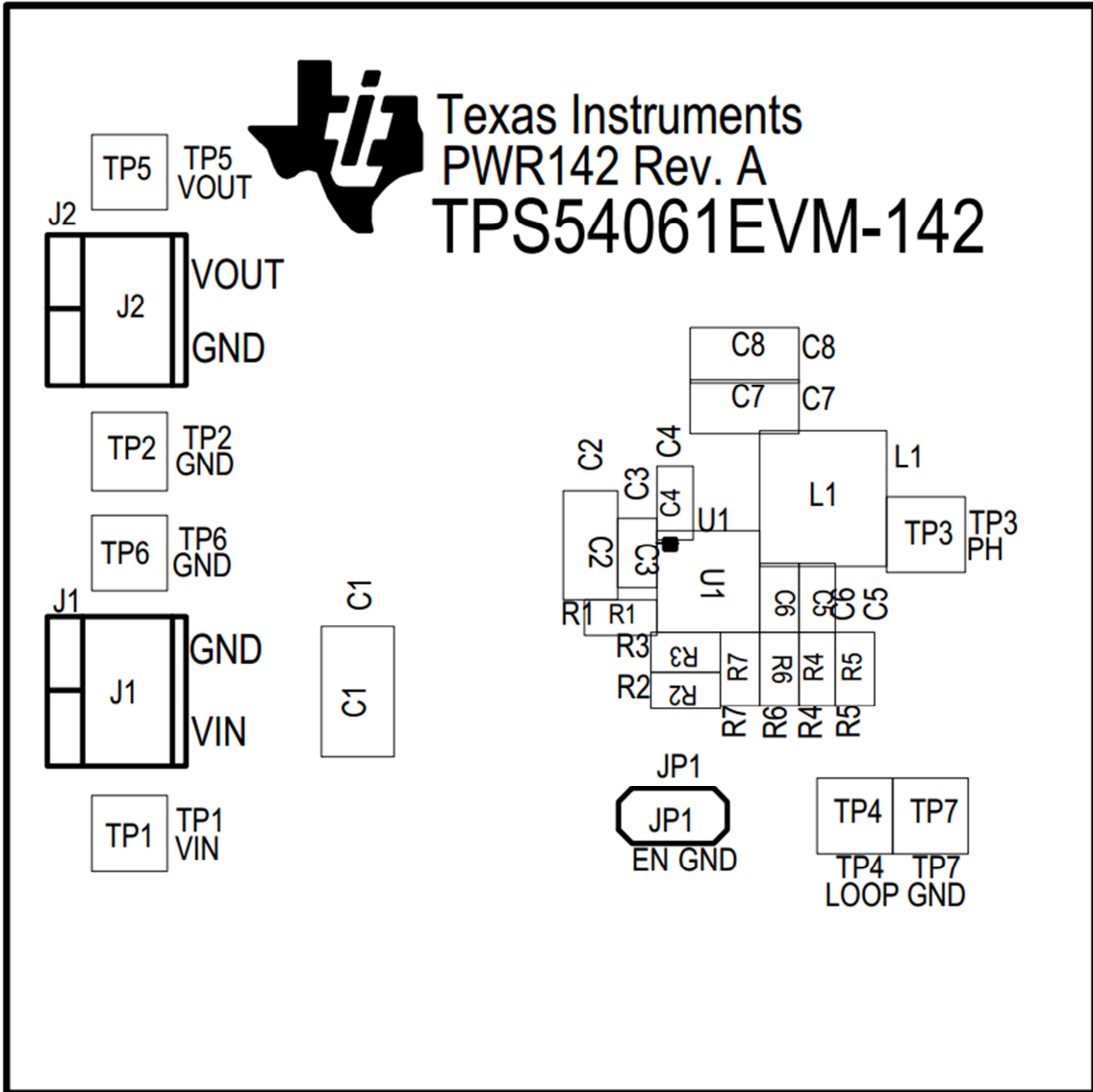
Figure 18. TPS54061EVM-142 Top Assembly and Silkscreen
