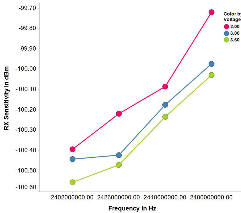
Figure 3. Sensitivity vs. Frequency and Power Supply Voltage for IEEE 802.15.4 PHY mode
