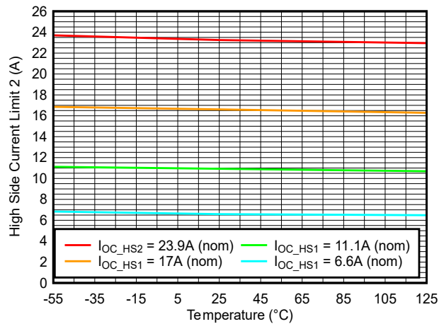
Figure 7-41. High-Side Current Limit Threshold 2 ( I_{OC\_HS2} ) vs Temperature
