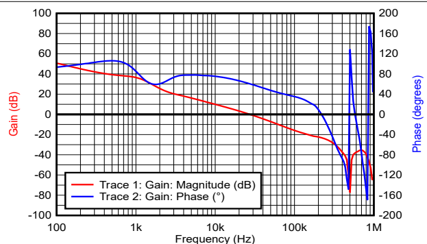
Figure 10-4. Bode Plot
