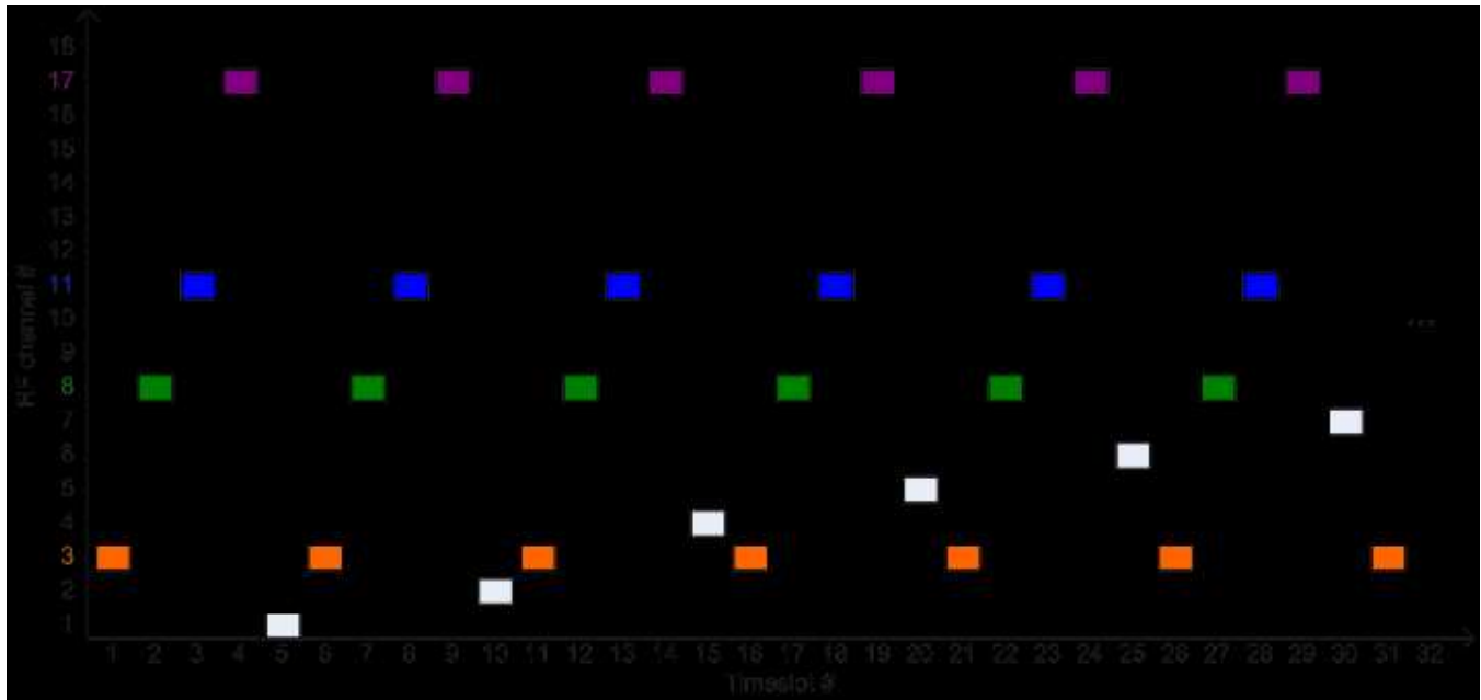
Figure 2. Example of AFH Hop Sequence
