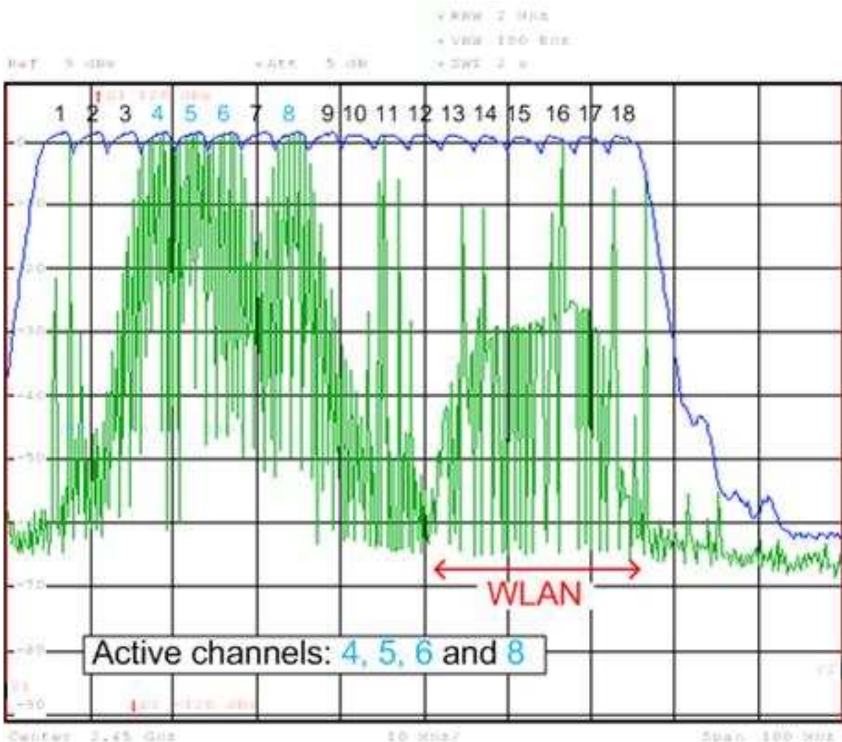
Figure 8. Adaptive Frequency Hopping in Practice
