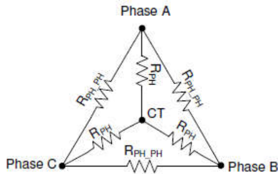
Figure 6-2. Resistance Measurement
