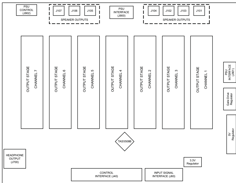
Figure 1-2. Physical Structure for TAS5508-5142K7EVM (Rough Outline)
