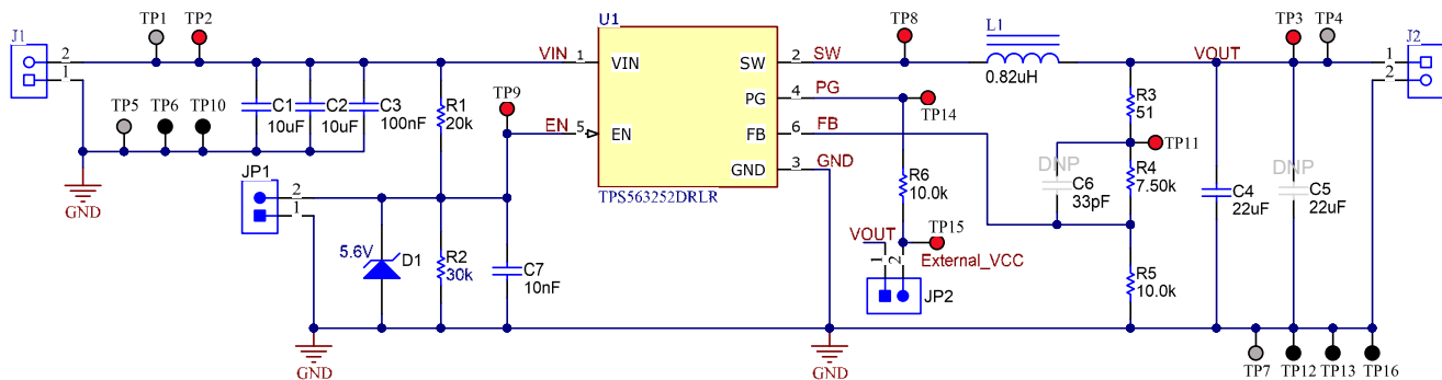
Figure 6-1. TPS563252EVM Schematic Diagram
