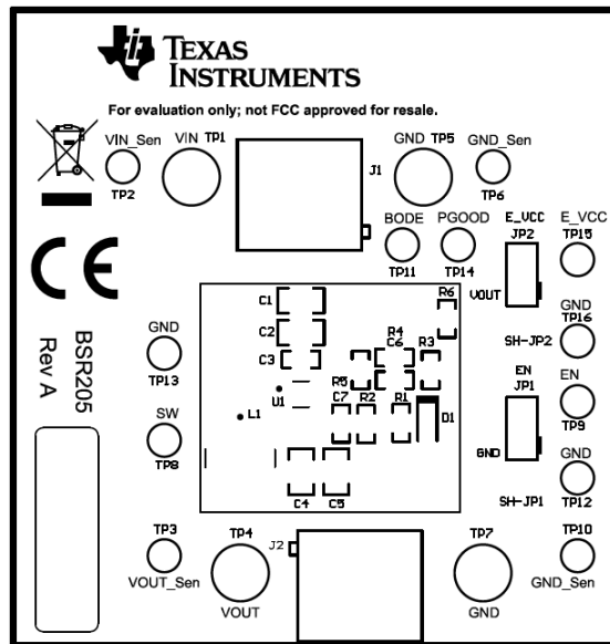
Figure 5-1. TPS563252EVM Top Assembly
