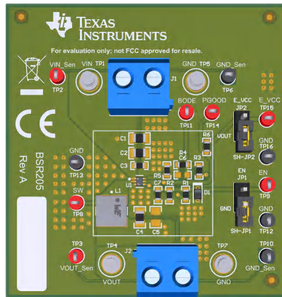
Figure 4-1. TPS563252EVM Connectors and Jumpers Placement
