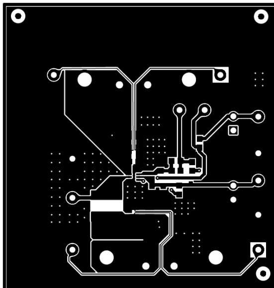
Figure 5-2. TPS563252EVM Top Layer
