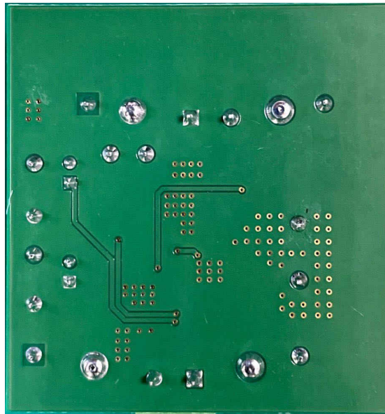
Figure 5-5. TPS563252EVM Board (Bottom View)
