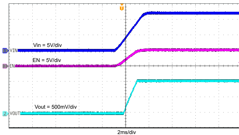
Figure 4-10. TPS563252EVM Start-Up Relative to V_{IN}
