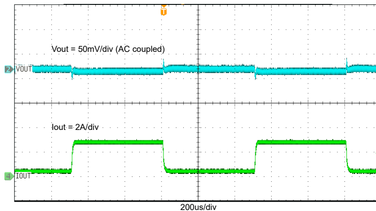
Figure 4-9. TPS563257EVM Load Transient Response, 10% to 90% (0.3 A to 2.7 A) Load Step
