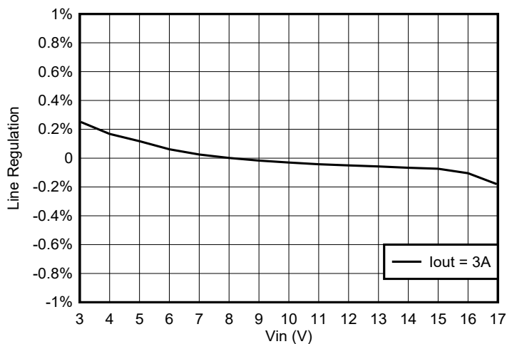
Figure 4-7. TPS563257EVM Line Regulation
