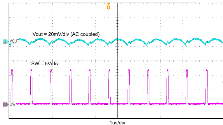
Figure 4-16. TPS563257EVM Output Voltage Ripple, I_{OUT} = 0.01\text{ A}
