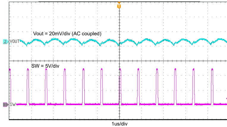
Figure 4-14. TPS563252EVM Output Voltage Ripple, I_{OUT} = 3\text{ A}
