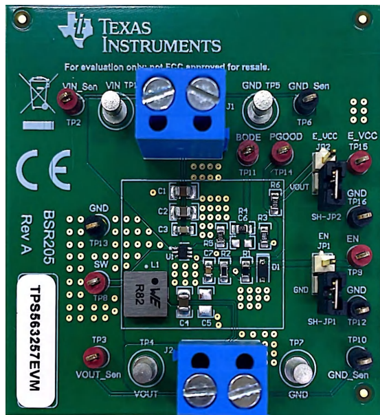
Figure 5-4. TPS563252EVM Board (Top View)
