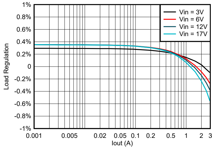
Figure 4-4. TPS563252EVM Load Regulation
