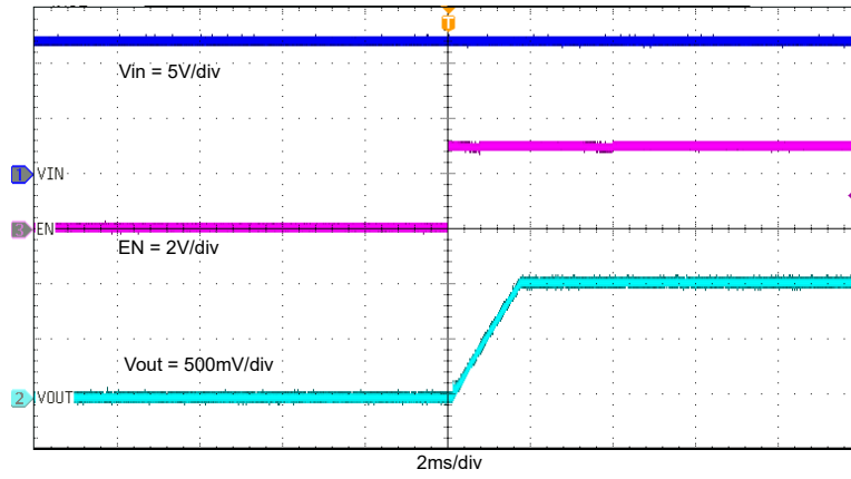
Figure 4-11. TPS563252EVM Start-Up Relative to EN
