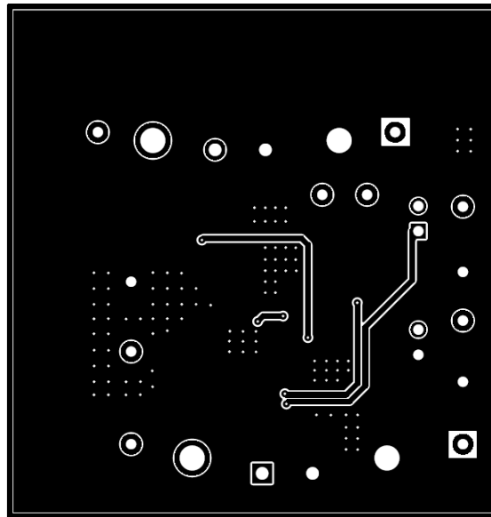
Figure 5-3. TPS563252EVM Bottom Layer
