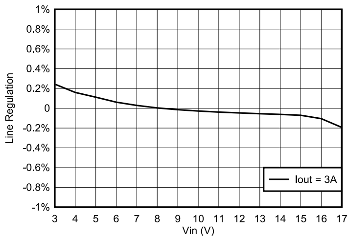
Figure 4-6. TPS563252EVM Line Regulation
