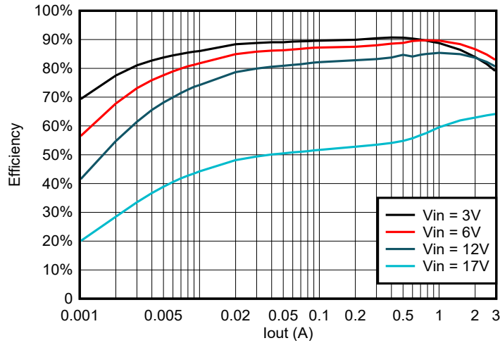
Figure 4-2. TPS563252EVM Efficiency
