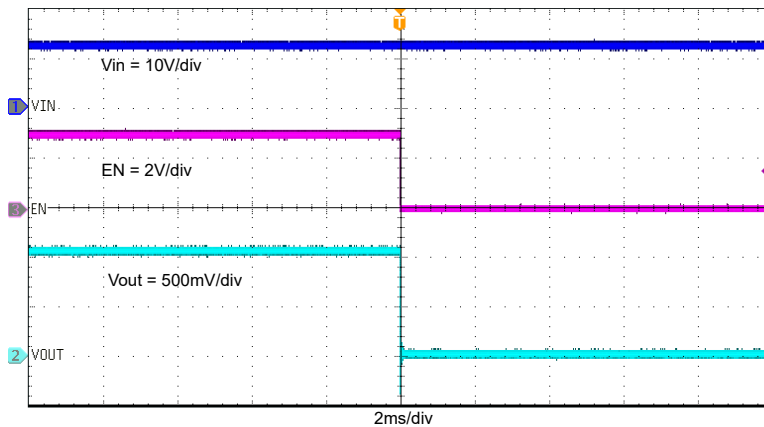
Figure 4-13. TPS563252EVM Shutdown Relative to EN
