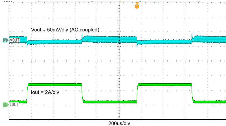
Figure 4-8. TPS563252EVM Load Transient Response, 10% to 90% (0.3 A to 2.7 A) Load Step
