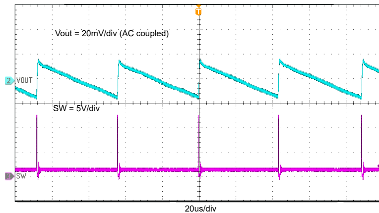
Figure 4-15. TPS563252EVM Output Voltage Ripple, I_{OUT} = 0.01\text{ A}
