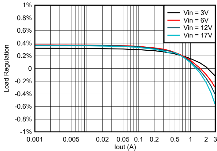
Figure 4-5. TPS563257EVM Load Regulation
