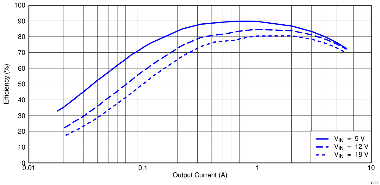
Figure 4-2. TPS54525EVM-608 Light Load Efficiency
