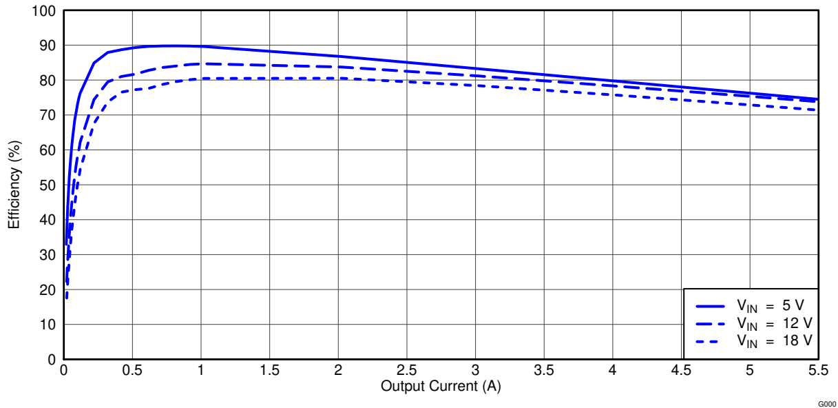
Figure 4-1. TPS54525EVM-608 Efficiency
