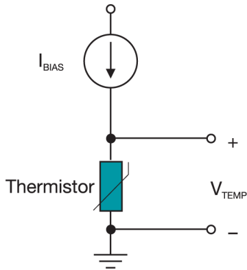
Figure 3. Thermistor Biased with a Constant Current Source.
