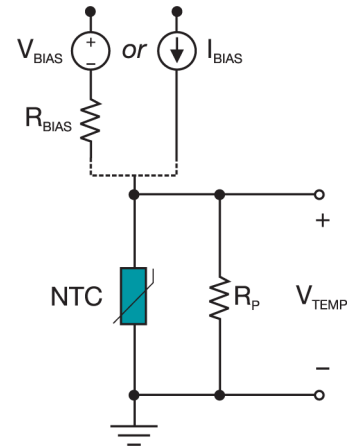
Figure 5. An NTC with a Parallel Resistor to Linearize V_{TEMP} .
