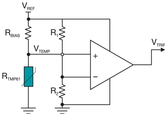
Figure 4. Using a Thermistor plus Comparator for Threshold Detection.
