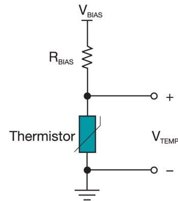
Figure 2. Thermistor Placed in a Voltage Divider Configuration.
