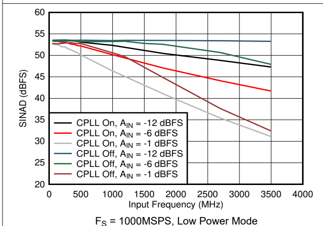
Figure 5-77. SINAD vs Input Frequency, CPLL and Input Amplitude
