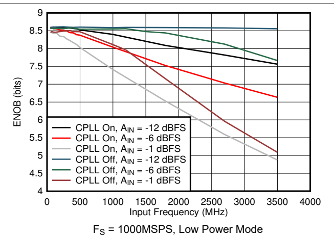
Figure 5-78. ENOB vs Input Frequency, CPLL and Input Amplitude
