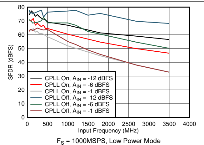
Figure 5-76. SFDR vs Input Frequency, CPLL and Input Amplitude
