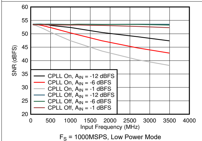
Figure 5-75. SNR vs Input Frequency, CPLL and Input Amplitude
