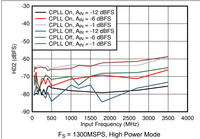
Figure 5-73. HD2 vs Input Frequency, CPLL and Input Amplitude
