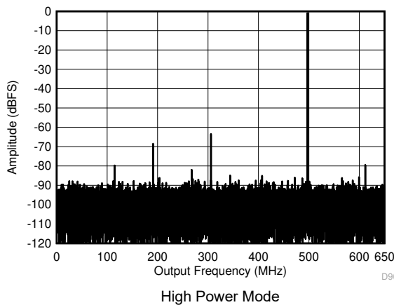
Figure 5-5. Single Tone FFT at 497 MHz and -1 dBFS
