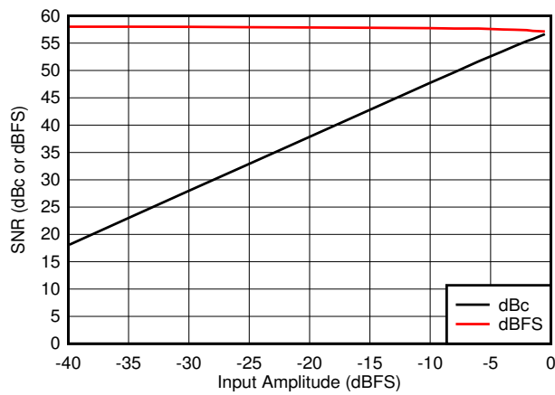
Figure 5-35. SNR vs A_{IN} F_{IN} = 100\text{MHz} , Low power mode
