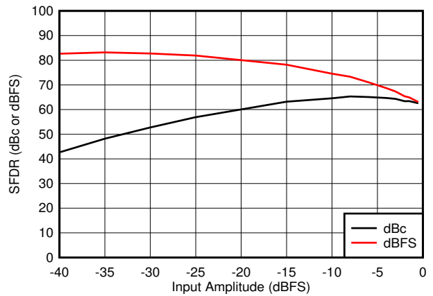
Figure 5-34. SFDR vs A_{IN} F_{IN} = 100\text{MHz} , Low power mode
