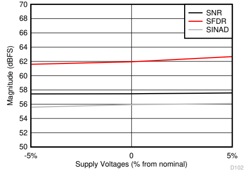
All supplies changed together, low power mode, F_S = 1000\text{MSPS} Figure 5-62. SNR, SFDR and SINAD vs Supply Voltages
