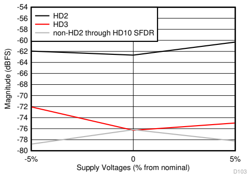
All supplies changed together, low power mode, F_S = 1000\text{MSPS} Figure 5-63. HD2, HD3 and Worst non-HD Spur vs Supply Voltage
