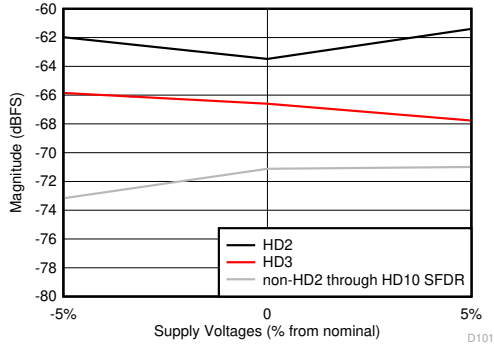
All supplies changed together, high power mode Figure 5-61. HD2, HD3 and Worst non-HD Spur vs Supply Voltage
