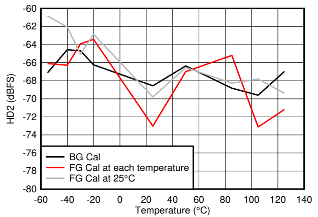
Figure 5-66. HD2 vs Temperature
