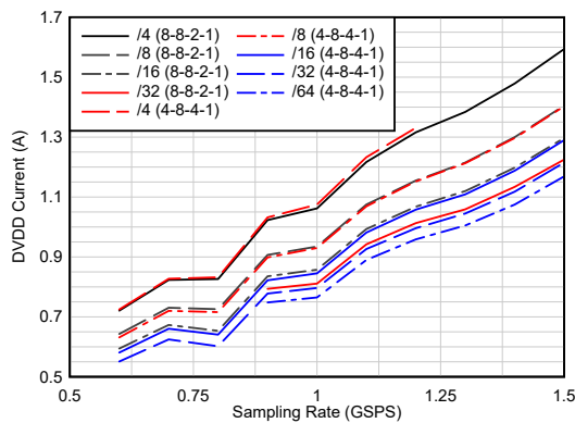
Figure 6-51. Current vs Sampling Rate vs Complex Decimation
