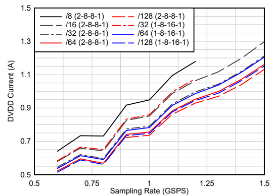
Figure 6-52. Current vs Sampling Rate vs Complex Decimation
