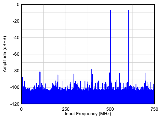
IMD3 = 72 dBc A_{IN} = -7\text{ dBFS/tone} , 2x AVG, Dither = DIS
