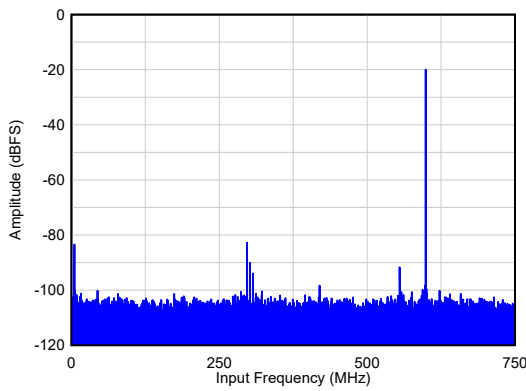
Figure 6-19. Single Tone FFT at F_{IN} = 900\text{ MHz}
