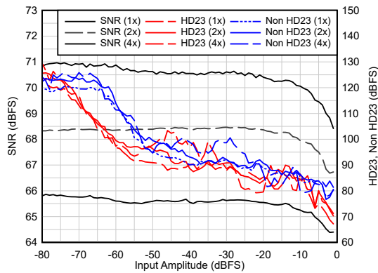
Figure 6-31. Dither Spur vs A_{IN}
