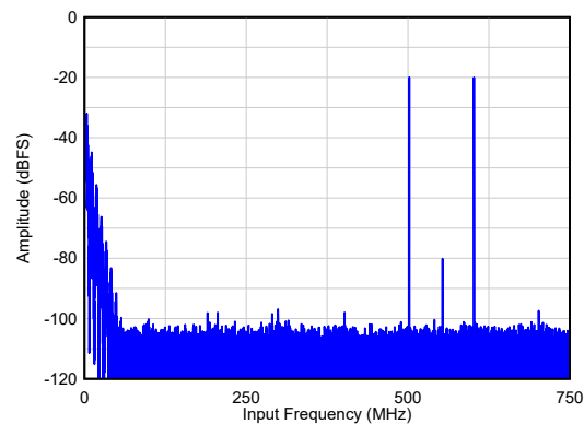
IMD3 = 77 dBc A_{IN} = -20\text{ dBFS/tone} , 2x AVG, Dither = EN
