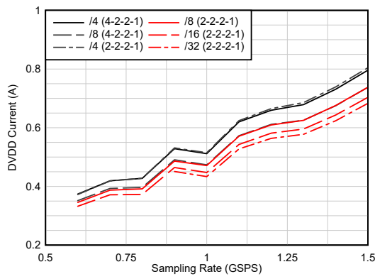
Figure 6-49. Current vs Sampling Rate vs Real Decimation
