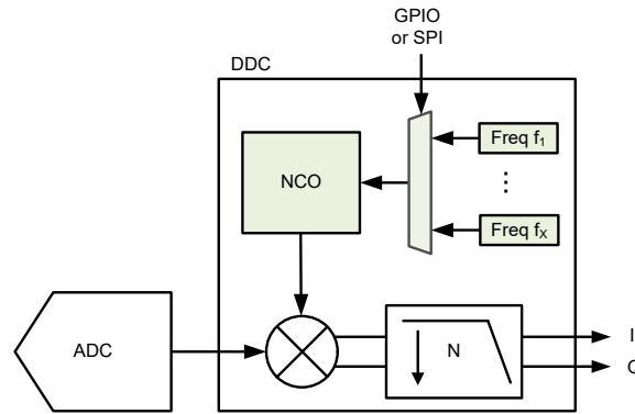
Figure 7-35. NCO Block Diagram
