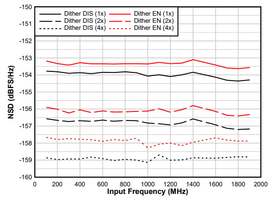
Figure 6-32. NSD Performance vs F_{IN}
