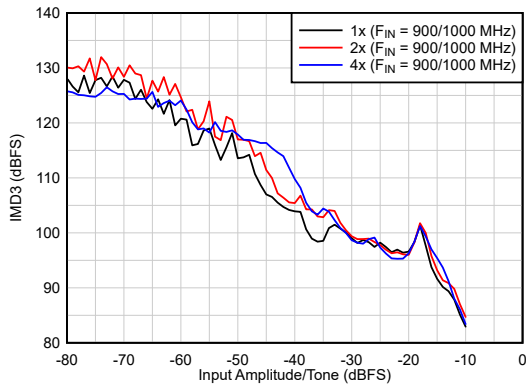
Figure 6-37. IMD3 Performance vs A_{IN}
