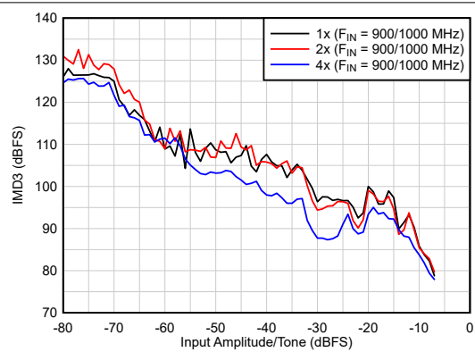
Figure 6-34. AC Performance vs A_{IN}
