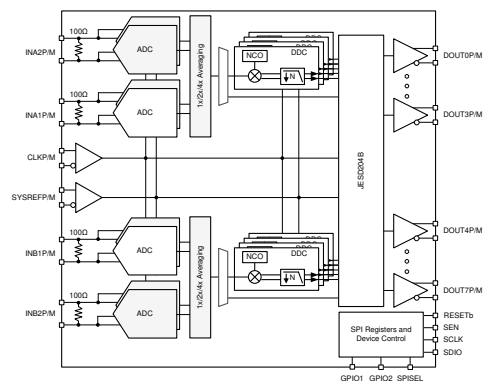
Block Diagram
