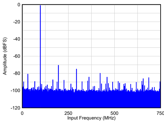
Figure 6-7. Single Tone FFT at F_{IN} = 1400\text{ MHz}
