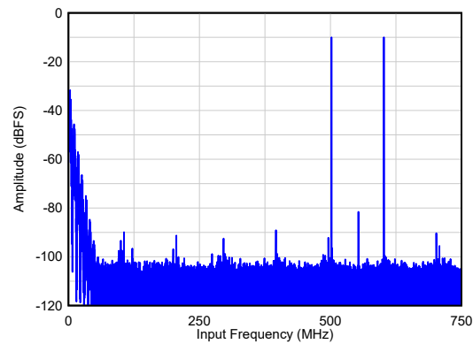
IMD3 = 79 dBc A_{IN} = -10\text{ dBFS/tone} , 2x AVG, Dither = EN
