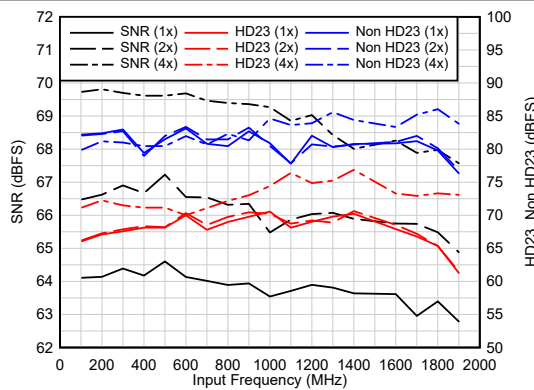
A_{IN} = -1\text{ dBFS} , Dither = DIS
