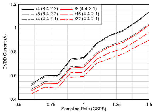
Figure 6-49. Current vs Sampling Rate vs Real Decimation
