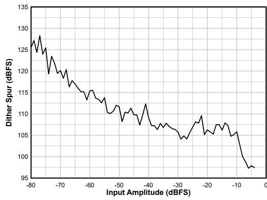
Figure 6-31. Dither Spur vs A_{IN}
