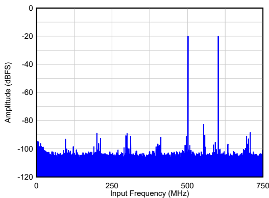
IMD3 = 63 dBc A_{IN} = -20\text{ dBFS/tone} , 2x AVG, Dither = DIS
