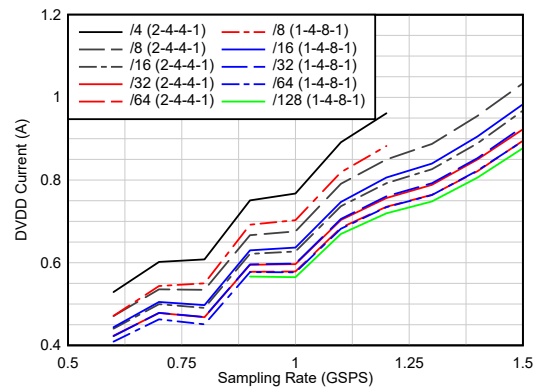
Figure 6-50. Current vs Sampling Rate vs Real Decimation
