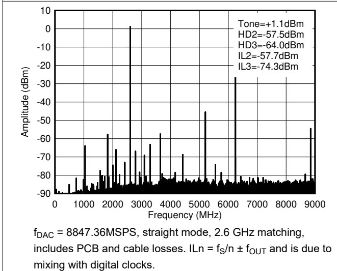
Figure 6-116. TX Single Tone (-1 dBFS) Output Spectrum at 2.6 GHz ( 0-f_{\text{DAC}} )
