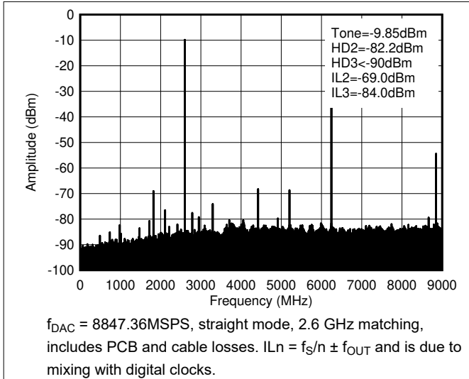
Figure 6-114. TX Single Tone (-12 dBFS) Output Spectrum at 2.6 GHz ( 0-f_{\text{DAC}} )
