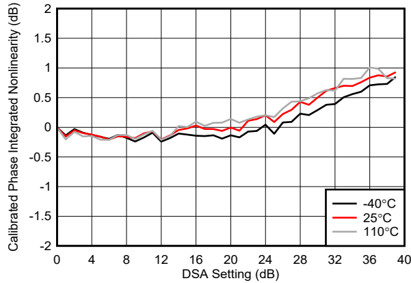
Figure 6-202. TX DSA Calibrated Phase Integrated Nonlinearity at 8.11 GHz
