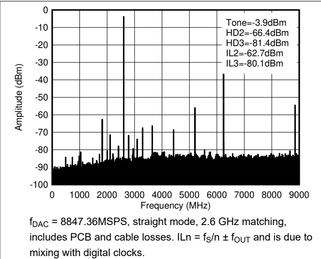
Figure 6-115. TX Single Tone (-6 dBFS) Output Spectrum at 2.6 GHz ( 0-f_{\text{DAC}} )
