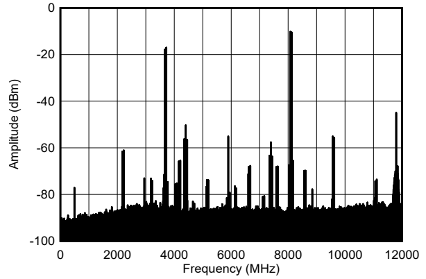
Figure 6-209. TX Dual Tone Output Spectrum at 8.11 GHz
