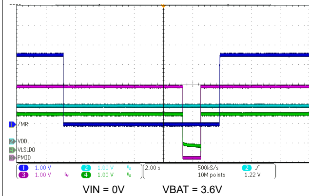
Figure 8-6. HW Reset on MR Long Button Press
