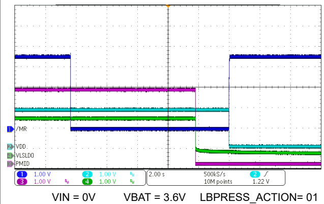
Figure 8-7. Ship Mode Entry with MR Long Button Press
