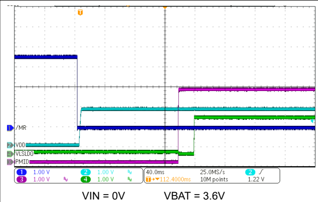
Figure 8-5. Power Up from Ship Mode with MR Press
