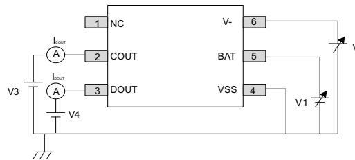
Figure 7-6. Test Circuit 4
