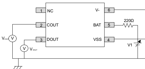
Figure 7-3. Test Circuit 1
