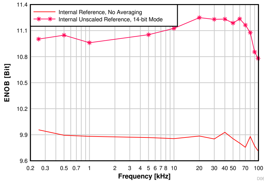
Figure 8-25. ENOB vs. Input Frequency
