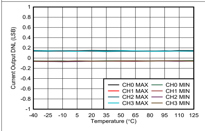
Figure 6-39. Current Output DNL vs Temperature
