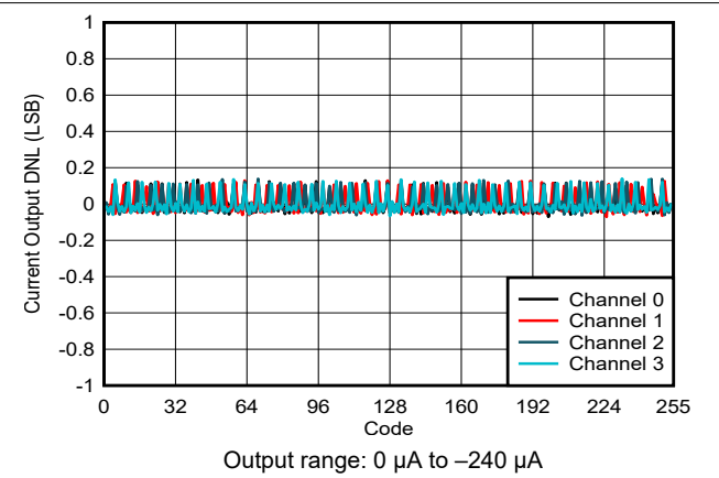
Figure 6-38. Current Output DNL vs Digital Input Code
