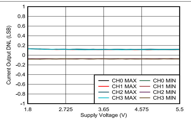
Figure 6-40. Current Output DNL vs Supply Voltage
