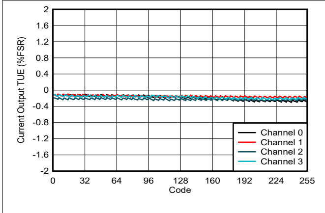
Figure 6-41. Current Output TUE vs Digital Input Code
