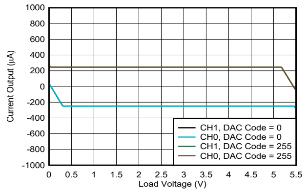
Figure 6-41. Current Output vs Load Voltage
