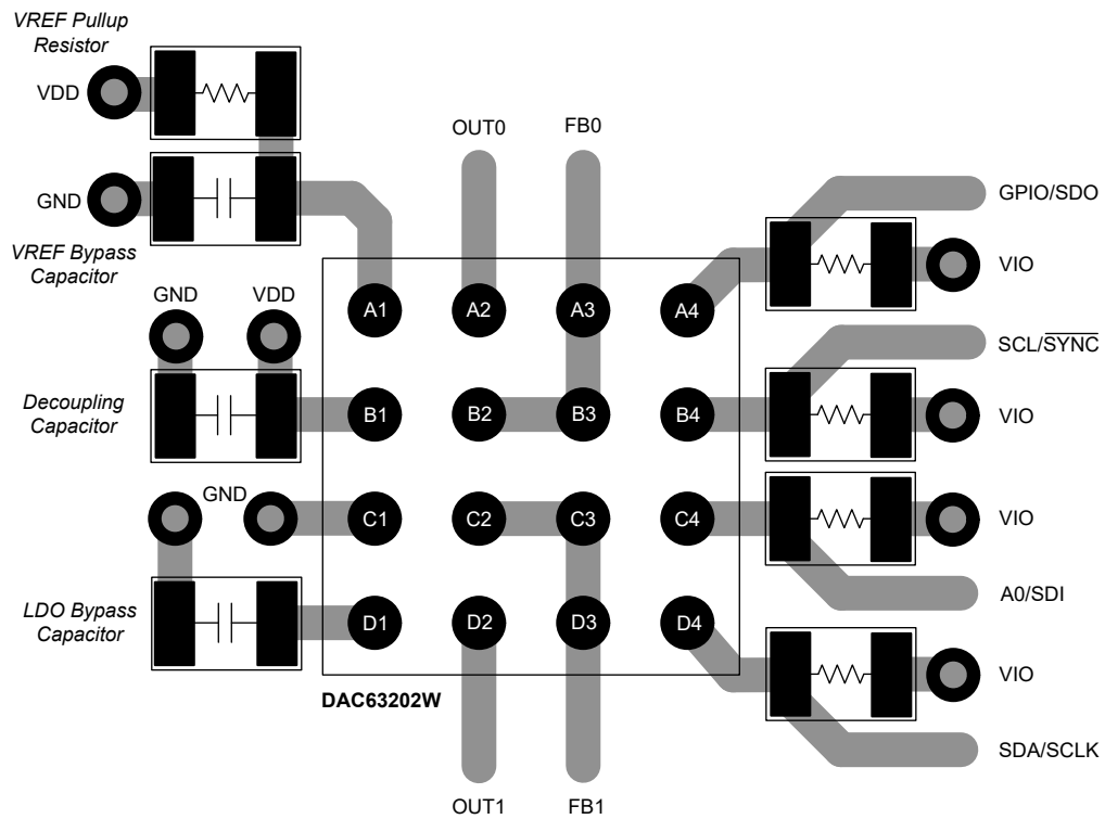
Figure 8-4. Layout Example
