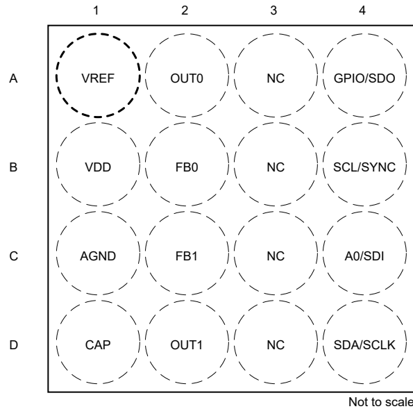
Figure 5-1. YBH (16-pin DSBGA) Package, Top View
