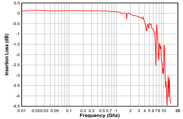
Figure 5-8. Insertion Loss
