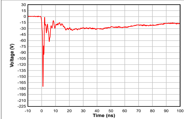
Figure 5-7. -8kV Clamped IEC Waveform
