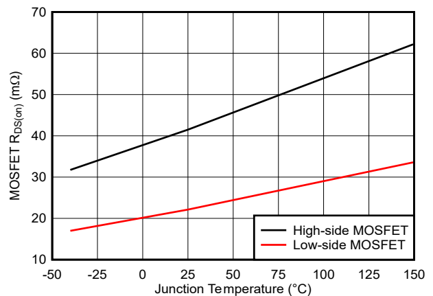
Figure 6-6. High-Side and Low-Side MOSFET R_{DS(on)}
