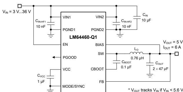
Typical Schematic
