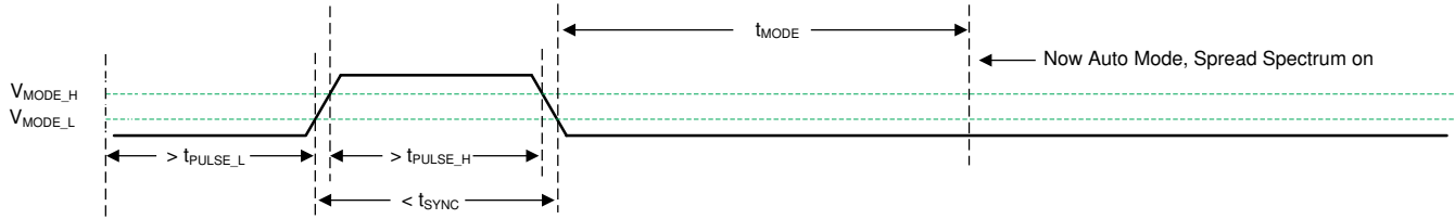
Figure 7-10. Transition from SYNC Mode to AUTO Mode
