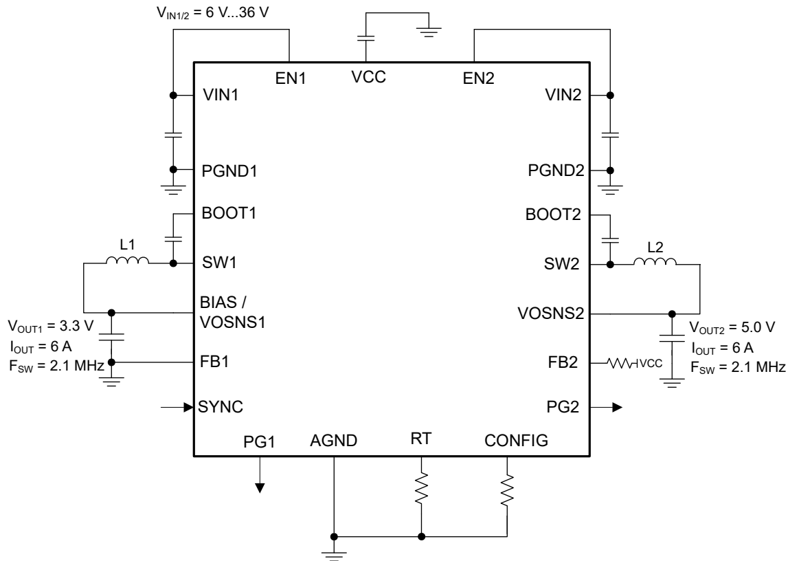
Figure 8-2. Example Application Circuit - 2.1-MHz Dual Fixed Output
