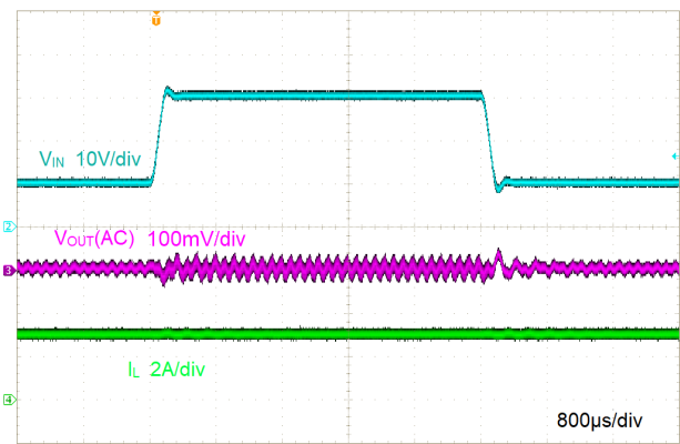
Figure 8-7. Line Transient
