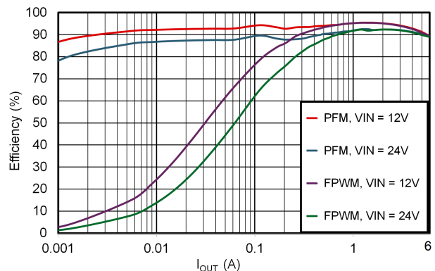
Efficiency vs Output Current V_{\text{OUT}} = 5\text{V} , 400kHz
