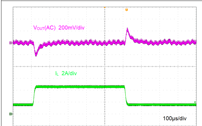
Figure 8-6. Load Transient
