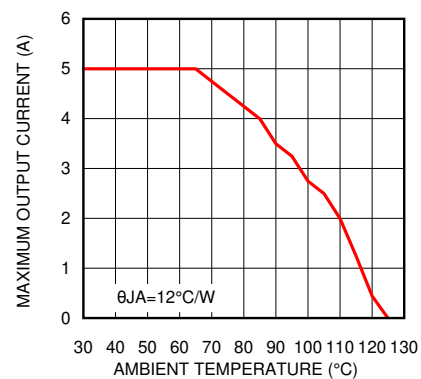
Figure 7-5. Thermal Derating Curve
