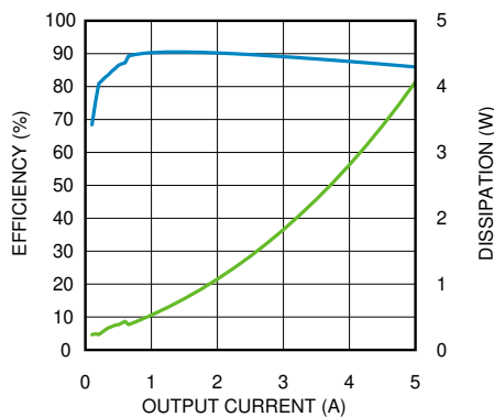
Figure 7-4. Efficiency
