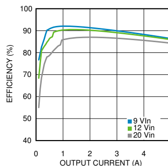
Efficiency 5-V Output Current at 25^{\circ}\text{C} Ambient
