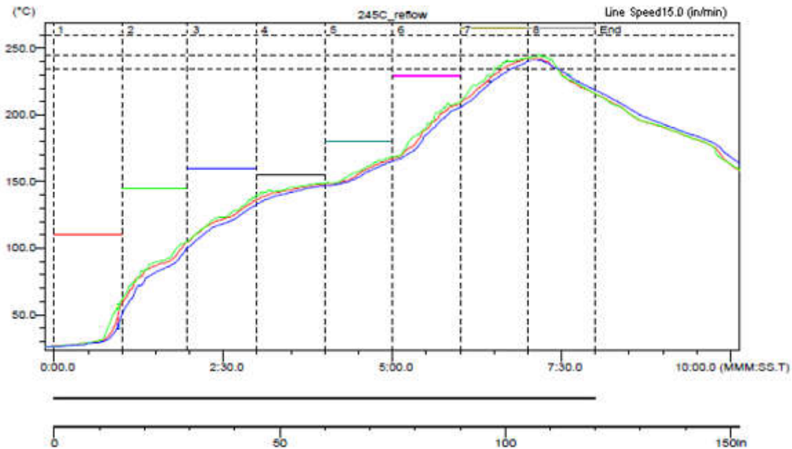
Figure 9-5. Sample Reflow Profile
