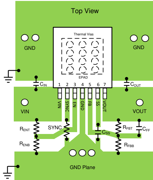
Figure 9-2. PCB Layout Guide
