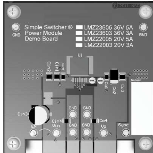
Figure 9-4. Bottom View Demonstration Board
