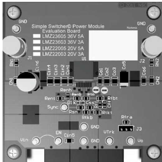
Figure 9-3. Top View Evaluation Board – See AN-2085 SNVA457
