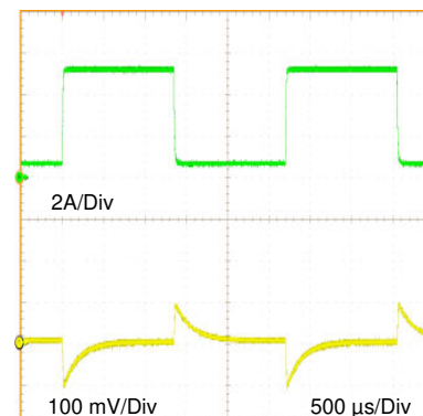
Figure 5-40. Output Ripple
