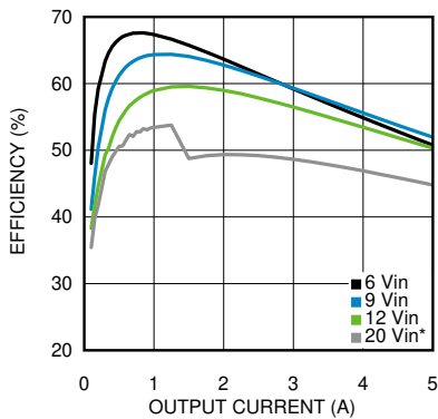
Figure 5-35. Efficiency 0.8-V at 85°C Ambient
