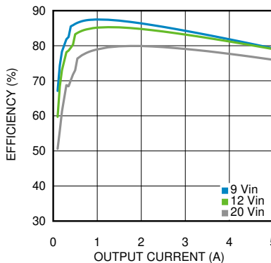
Figure 5-23. Efficiency 3.3-V Output at 85°C Ambient
