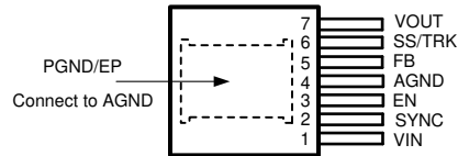
Figure 4-1. NDW Package 7-Pin Top View
