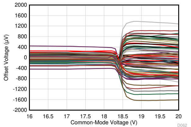
T_A = -40^\circ\text{C} Data from 74 amplifiers
