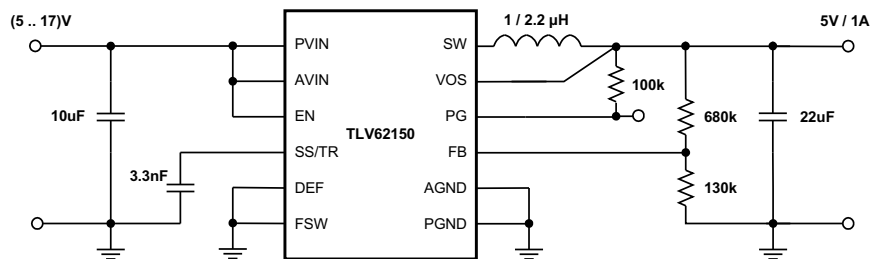
Figure 39. 5-V/1-A Power Supply
