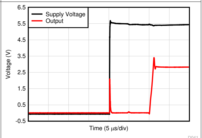
Figure 7-80. Turn-On Time
