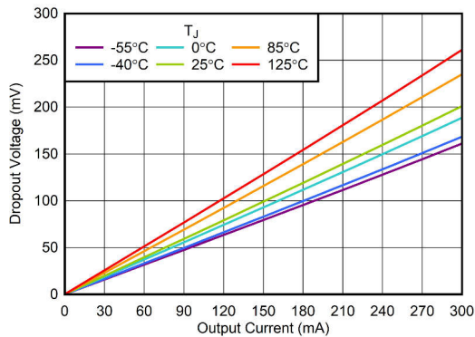
Figure 5-5. Dropout Voltage vs I_{OUT}
