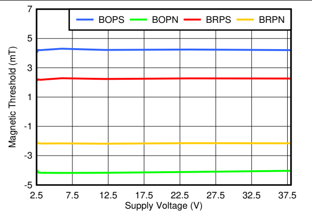
Figure 7-4. TMAG5123B Magnetic Thresholds vs Voltage
