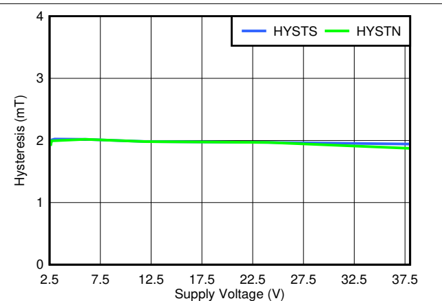
Figure 7-6. TMAG5123B Hysteresis vs Supply Voltage
