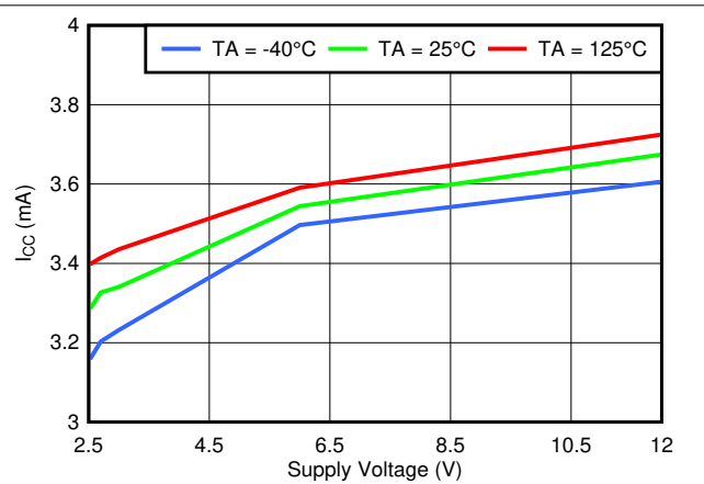
Figure 7-2. TMAG5123 I_{CC} vs Voltage
