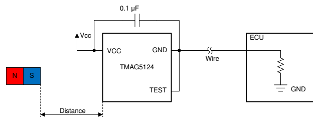
Typical Schematic
