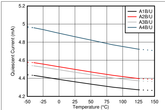
Figure 7-7. Quiescent Current vs. Temperature
