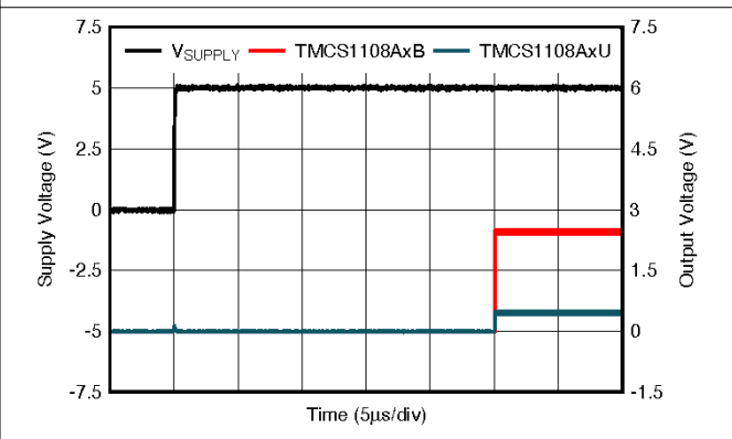
Figure 7-12. Startup Transient Response
