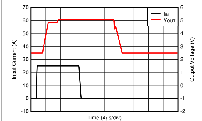
Figure 7-11. Current Overload Response
