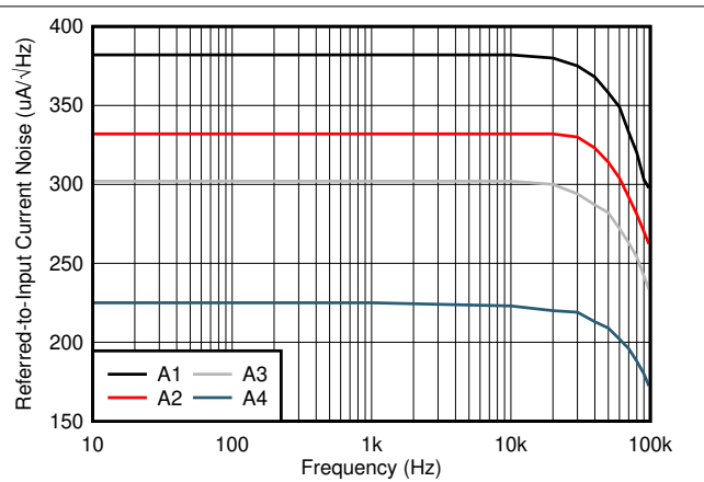
Figure 7-8. Input-Referred Noise vs. Frequency
