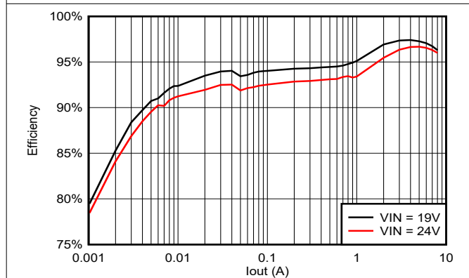
Figure 5-21. TPS56837 Efficiency, V_{out} = 12V , F_{sw} = 800kHz
