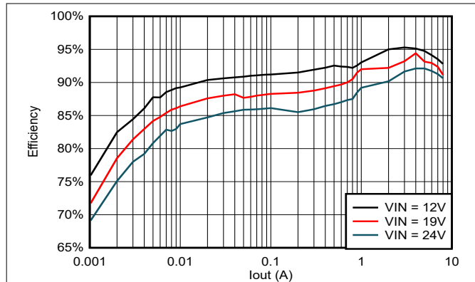
Figure 5-19. TPS56837 Efficiency, V_{out} = 5V , F_{sw} = 1200kHz
