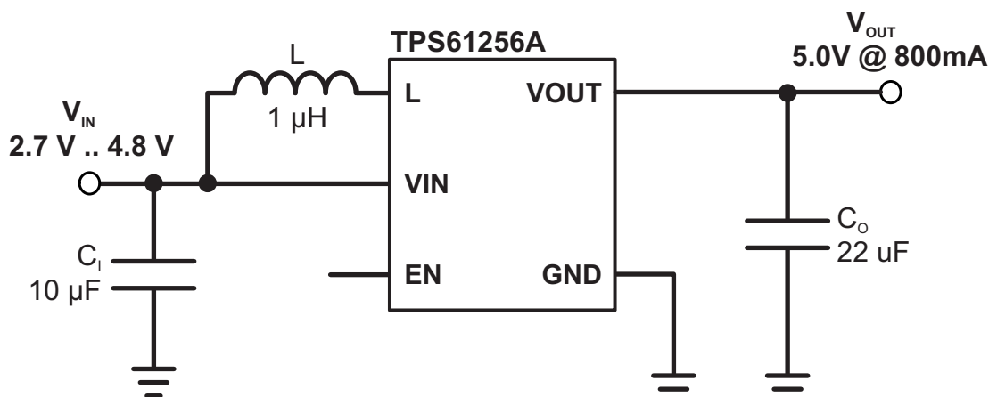
Figure 14. Typical Application
