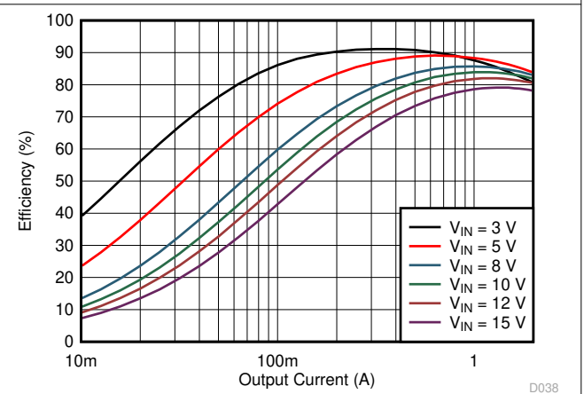
Figure 10-3. Efficiency vs Output Current
