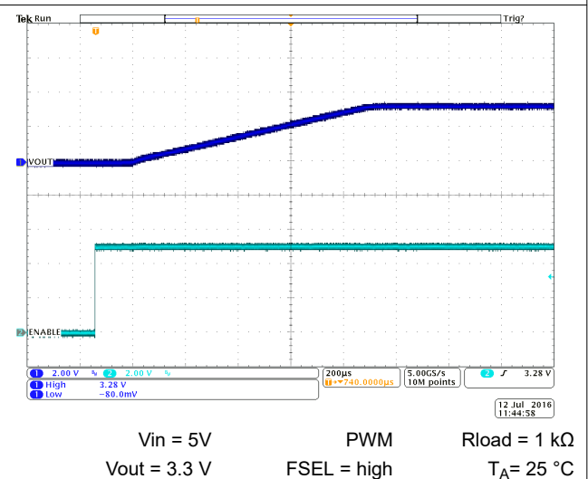
Figure 10-49. Start-Up Timing
