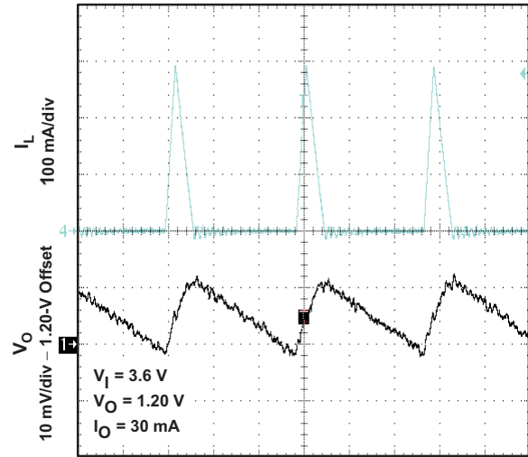
t – Time = 500 ns/div
