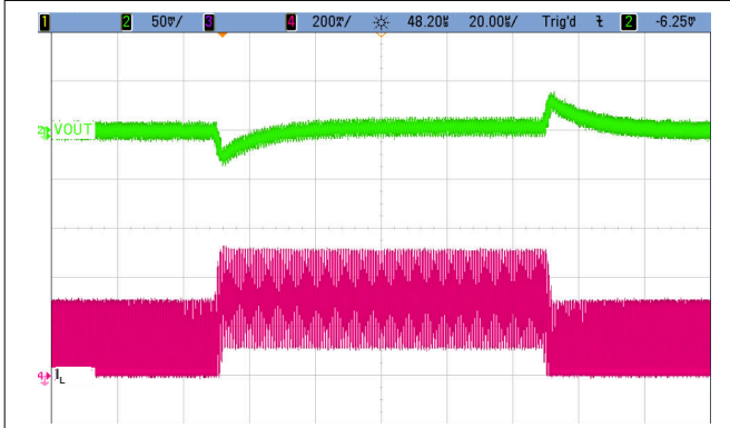
Figure 9-18. Load Transient Response; 100 mA to 290 mA
